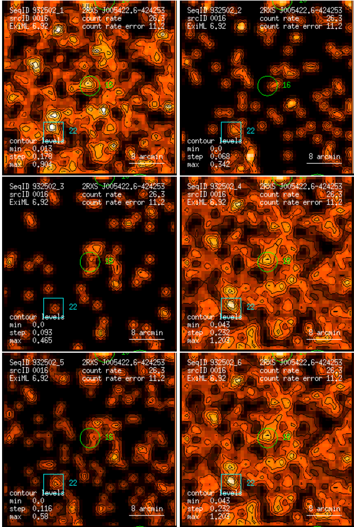
Figure 16: RASS 932502: detection 0016: band rate images, Gaussian filter: (1) PSPC channels 11 – 41, (2) 52 – 90, (3) 91 – 201, (4) 11 – 235, (5) 52 – 201, (6) 11 – 201. Broad band rates in counts/ks. Band rate contour levels in counts/ks/arcmin 2 .
