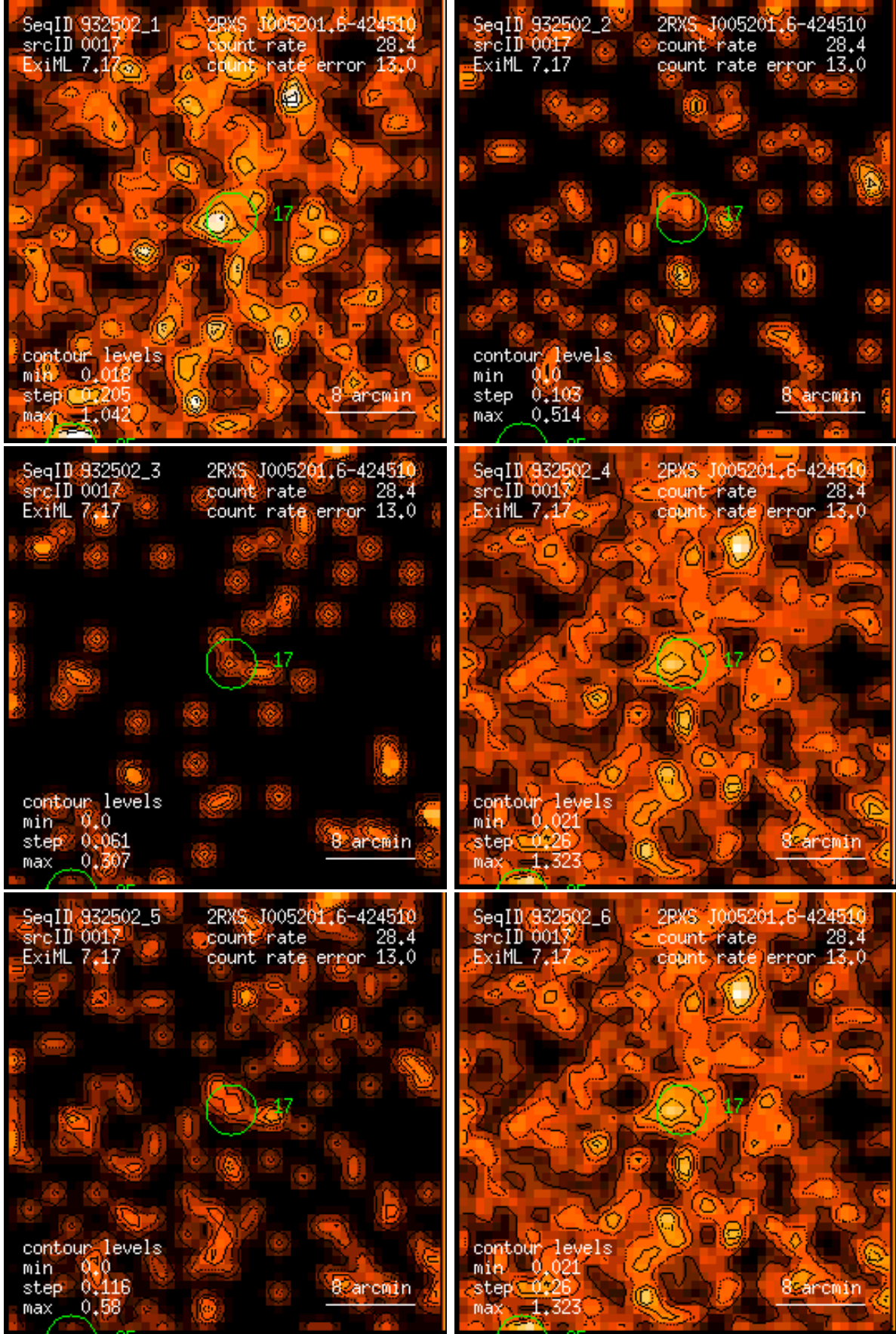
Figure 17: RASS 932502: detection 0017: band rate images, Gaussian filter: (1) PSPC channels 11 – 41, (2) 52 – 90, (3) 91 – 201, (4) 11 – 235, (5) 52 – 201, (6) 11 – 201. Broad band rates in counts/ks. Band rate contour levels in counts/ks/arcmin 2 .
