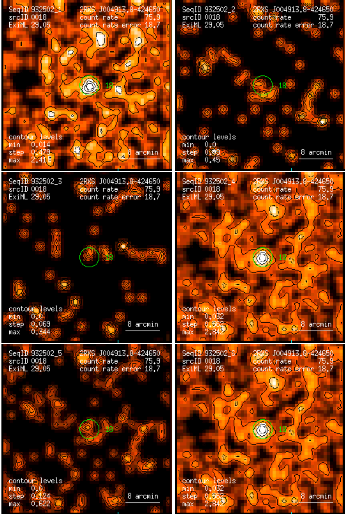
Figure 18: RASS 932502: detection 0018: band rate images, Gaussian filter: (1) PSPC channels 11 – 41, (2) 52 – 90, (3) 91 – 201, (4) 11 – 235, (5) 52 – 201, (6) 11 – 201. Broad band rates in counts/ks. Band rate contour levels in counts/ks/arcmin 2 .
