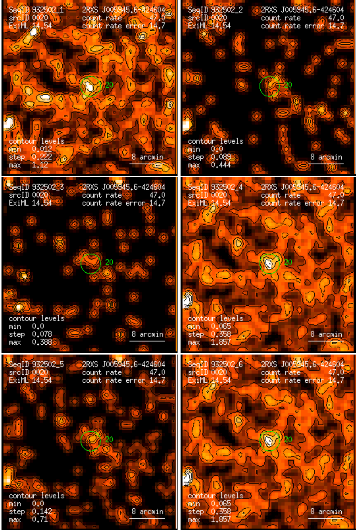
Figure 20: RASS 932502: detection 0020: band rate images, Gaussian filter: (1) PSPC channels 11 – 41, (2) 52 – 90, (3) 91 – 201, (4) 11 – 235, (5) 52 – 201, (6) 11 – 201. Broad band rates in counts/ks. Band rate contour levels in counts/ks/arcmin 2 .
