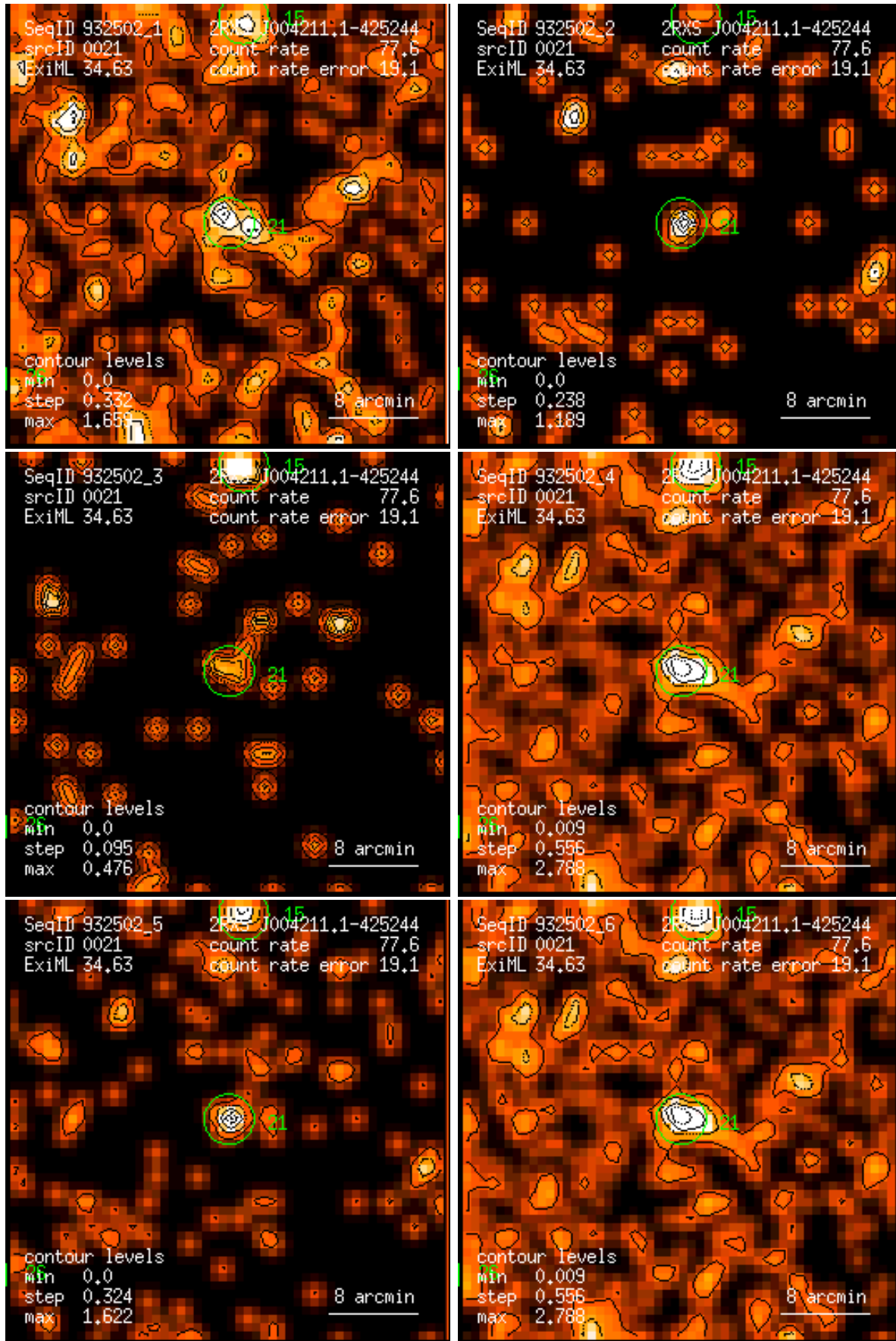
Figure 21: RASS 932502: detection 0021: band rate images, Gaussian filter: (1) PSPC channels 11 – 41, (2) 52 – 90, (3) 91 – 201, (4) 11 – 235, (5) 52 – 201, (6) 11 – 201. Broad band rates in counts/ks. Band rate contour levels in counts/ks/arcmin 2 .
