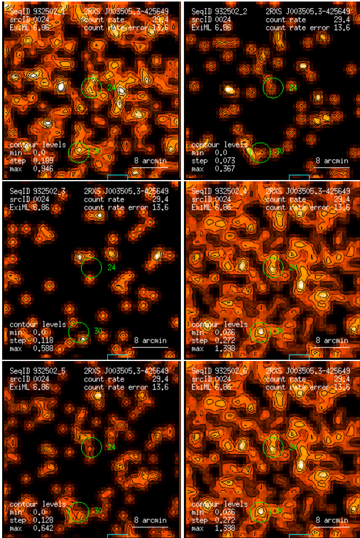
Figure 24: RASS 932502: detection 0024: band rate images, Gaussian filter: (1) PSPC channels 11 – 41, (2) 52 – 90, (3) 91 – 201, (4) 11 – 235, (5) 52 – 201, (6) 11 – 201. Broad band rates in counts/ks. Band rate contour levels in counts/ks/arcmin 2 .
