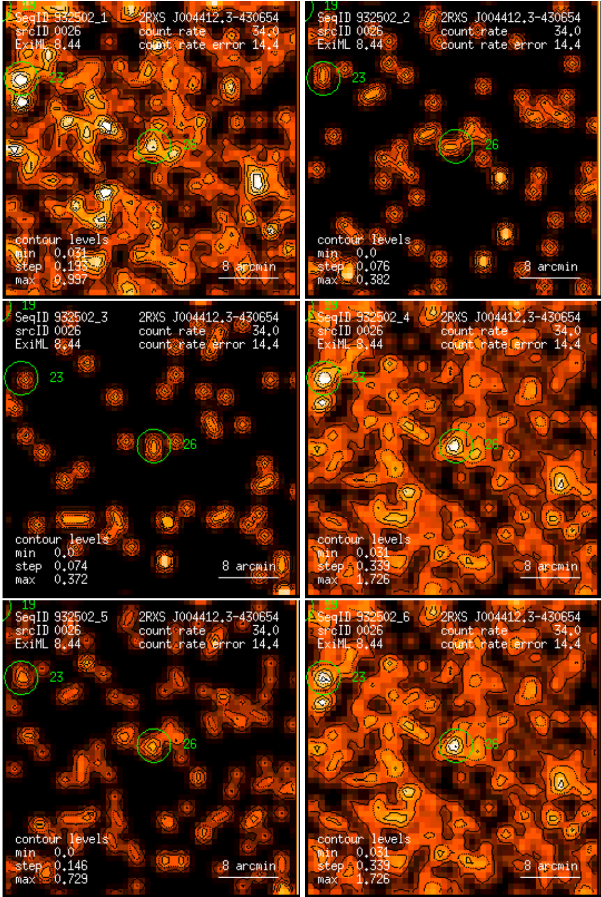
Figure 26: RASS 932502: detection 0026: band rate images, Gaussian filter: (1) PSPC channels 11 – 41, (2) 52 – 90, (3) 91 – 201, (4) 11 – 235, (5) 52 – 201, (6) 11 – 201. Broad band rates in counts/ks. Band rate contour levels in counts/ks/arcmin 2 .
