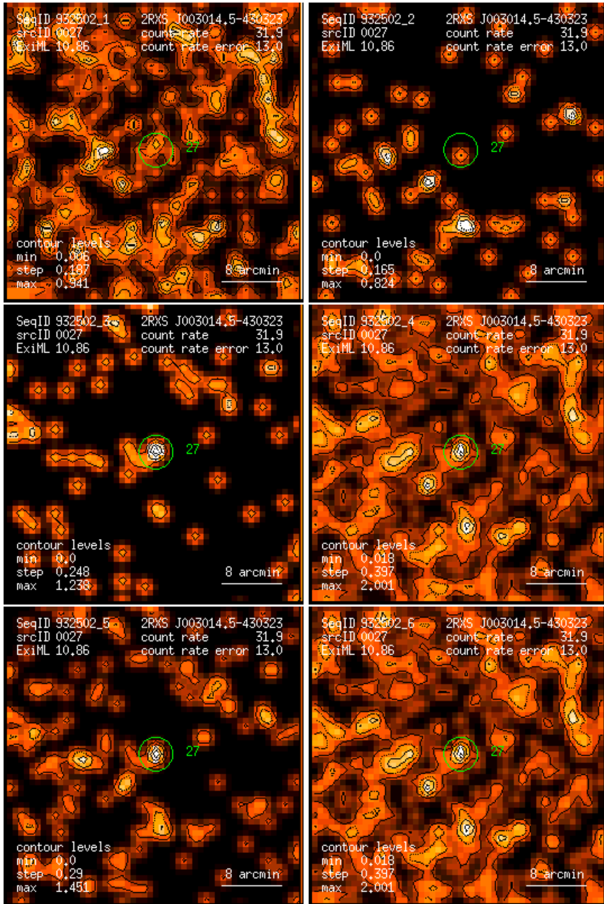
Figure 27: RASS 932502: detection 0027: band rate images, Gaussian filter: (1) PSPC channels 11 – 41, (2) 52 – 90, (3) 91 – 201, (4) 11 – 235, (5) 52 – 201, (6) 11 – 201. Broad band rates in counts/ks. Band rate contour levels in counts/ks/arcmin 2 .
