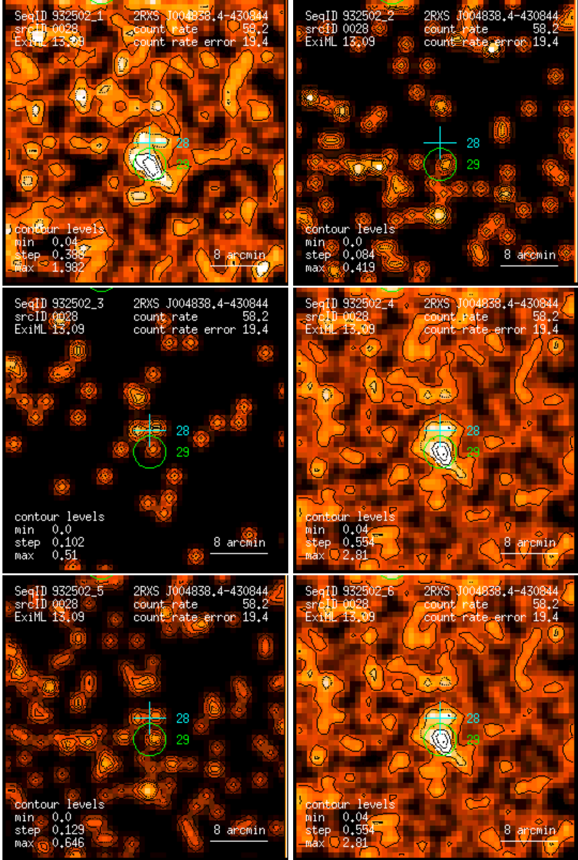
Figure 28: RASS 932502: detection 0028: band rate images, Gaussian filter: (1) PSPC channels 11 – 41, (2) 52 – 90, (3) 91 – 201, (4) 11 – 235, (5) 52 – 201, (6) 11 – 201. Broad band rates in counts/ks. Band rate contour levels in counts/ks/arcmin 2 .
