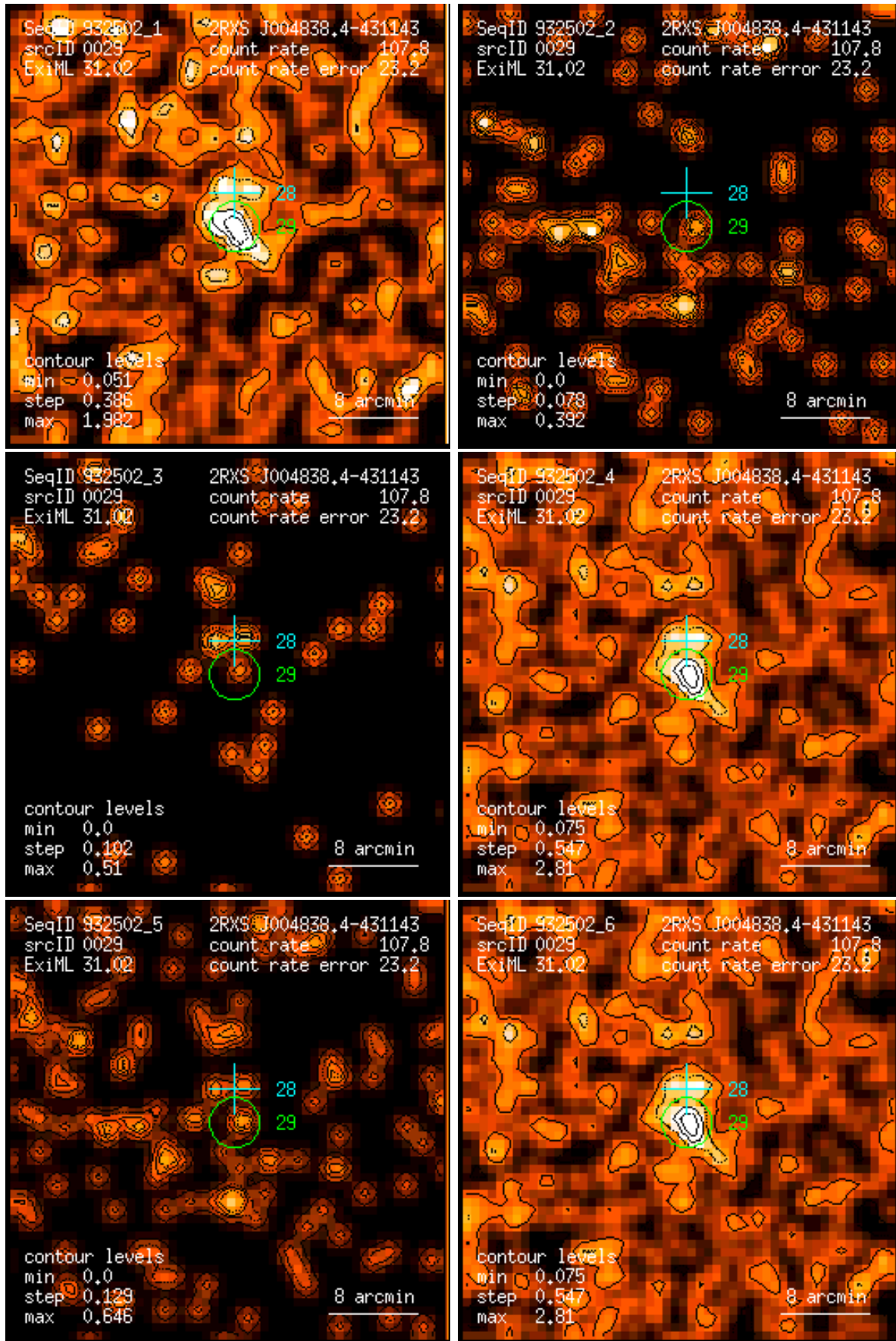
Figure 29: RASS 932502: detection 0029: band rate images, Gaussian filter: (1) PSPC channels 11 – 41, (2) 52 – 90, (3) 91 – 201, (4) 11 – 235, (5) 52 – 201, (6) 11 – 201. Broad band rates in counts/ks. Band rate contour levels in counts/ks/arcmin 2 .
