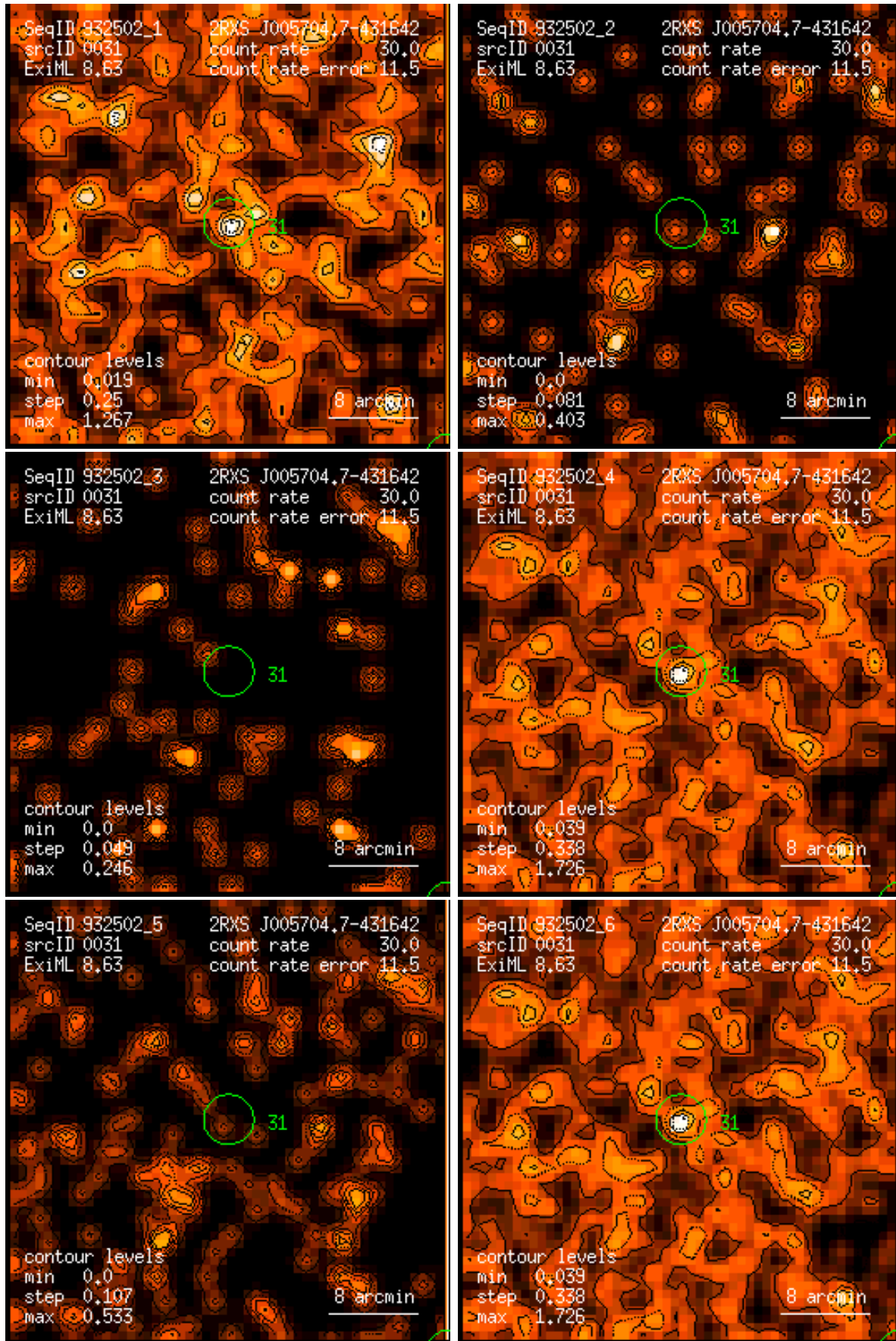
Figure 31: RASS 932502: detection 0031: band rate images, Gaussian filter: (1) PSPC channels 11 – 41, (2) 52 – 90, (3) 91 – 201, (4) 11 – 235, (5) 52 – 201, (6) 11 – 201. Broad band rates in counts/ks. Band rate contour levels in counts/ks/arcmin 2 .
