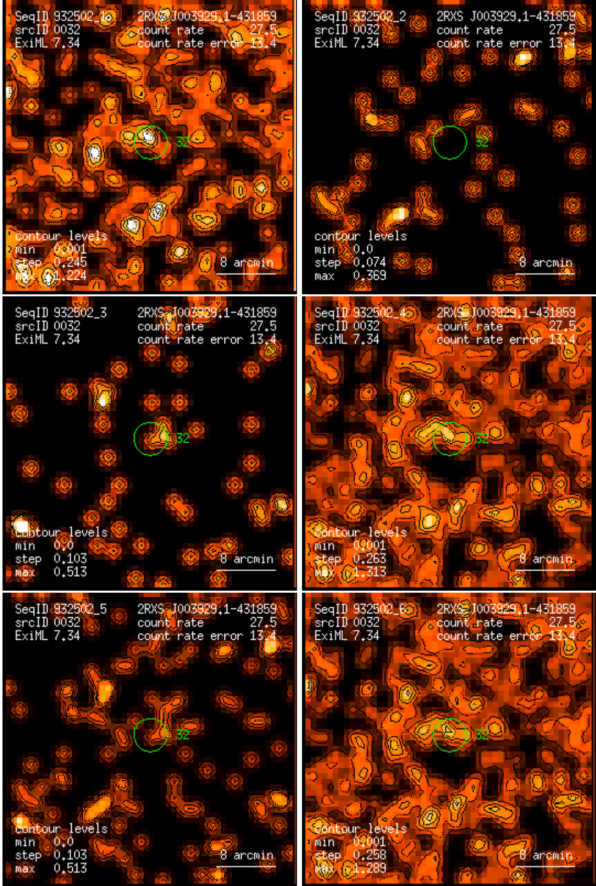
Figure 32: RASS 932502: detection 0032: band rate images, Gaussian filter: (1) PSPC channels 11 – 41, (2) 52 – 90, (3) 91 – 201, (4) 11 – 235, (5) 52 – 201, (6) 11 – 201. Broad band rates in counts/ks. Band rate contour levels in counts/ks/arcmin 2 .
