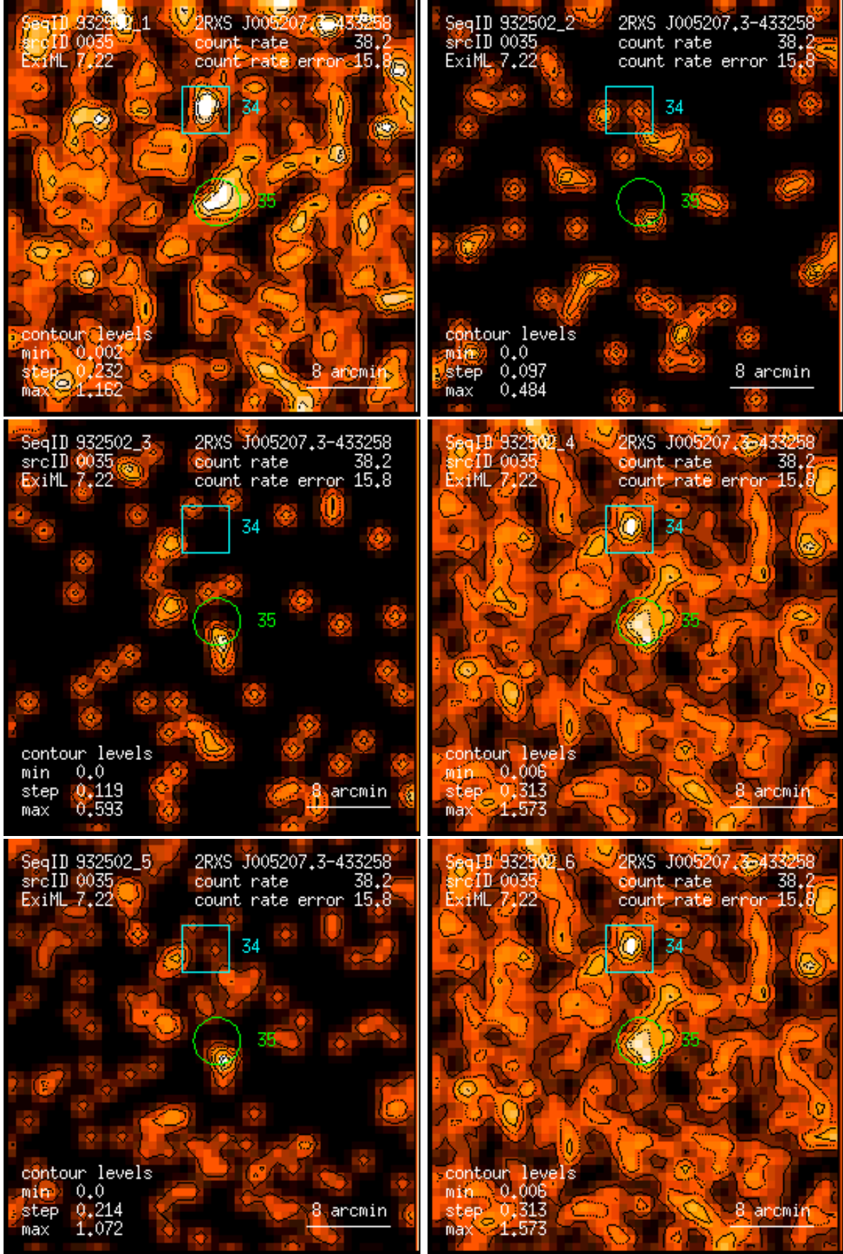
Figure 35: RASS 932502: detection 0035: band rate images, Gaussian filter: (1) PSPC channels 11 – 41, (2) 52 – 90, (3) 91 – 201, (4) 11 – 235, (5) 52 – 201, (6) 11 – 201. Broad band rates in counts/ks. Band rate contour levels in counts/ks/arcmin 2 .
