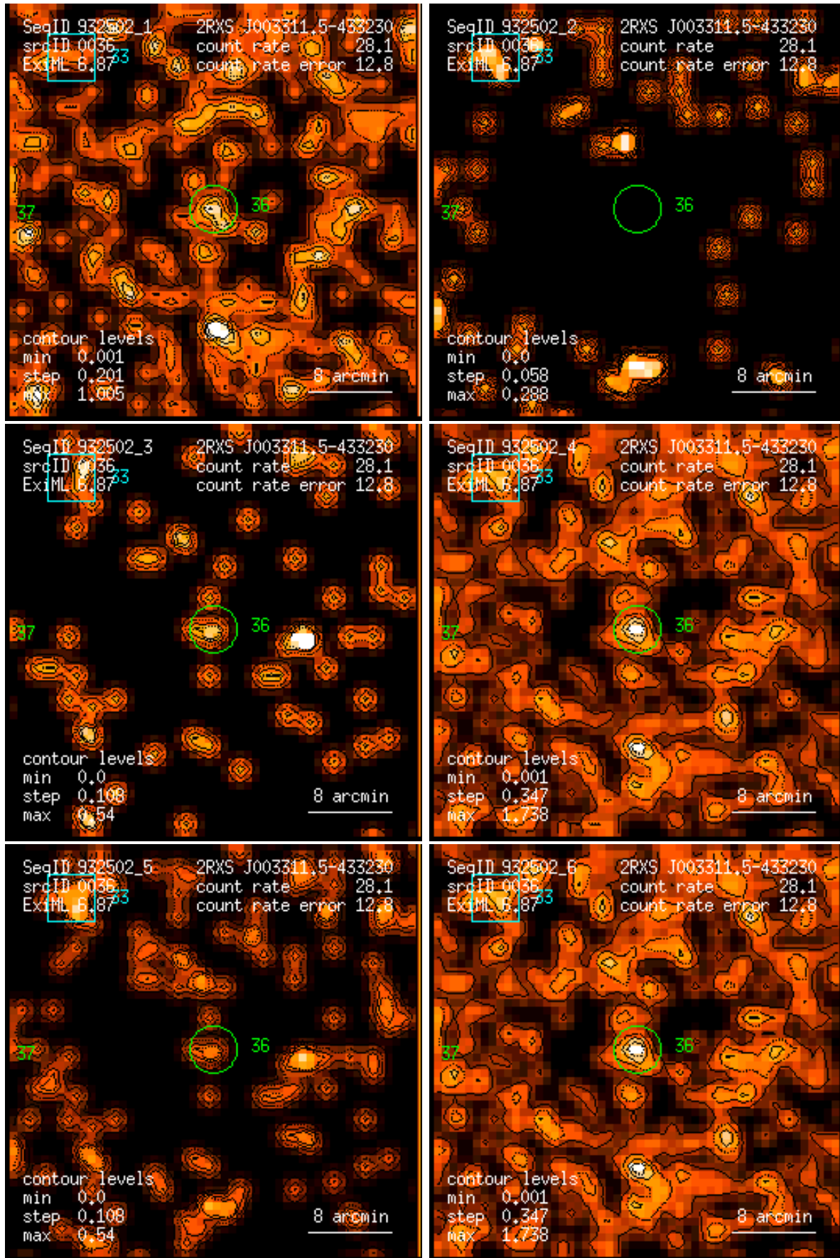
Figure 36: RASS 932502: detection 0036: band rate images, Gaussian filter: (1) PSPC channels 11 – 41, (2) 52 – 90, (3) 91 – 201, (4) 11 – 235, (5) 52 – 201, (6) 11 – 201. Broad band rates in counts/ks. Band rate contour levels in counts/ks/arcmin 2 .
