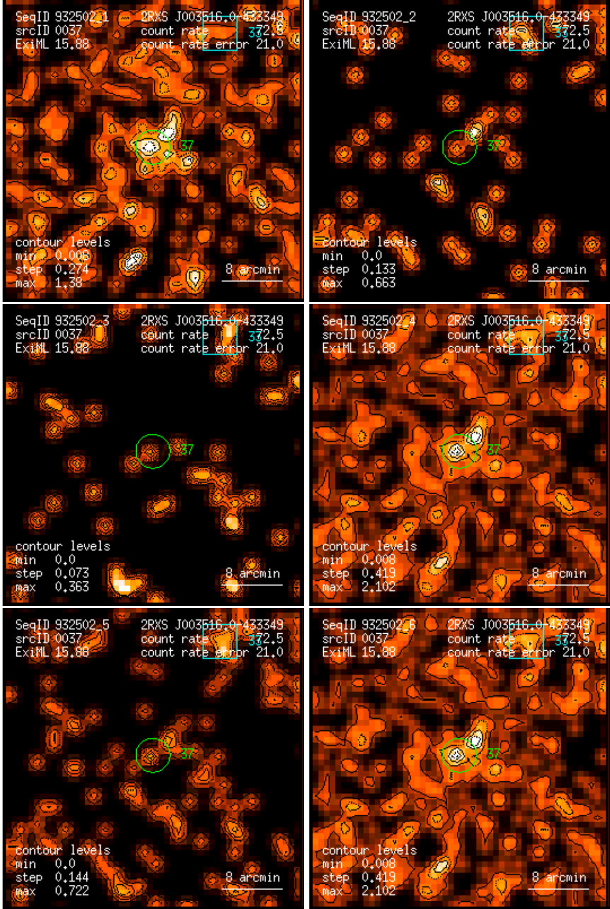
Figure 37: RASS 932502: detection 0037: band rate images, Gaussian filter: (1) PSPC channels 11 – 41, (2) 52 – 90, (3) 91 – 201, (4) 11 – 235, (5) 52 – 201, (6) 11 – 201. Broad band rates in counts/ks. Band rate contour levels in counts/ks/arcmin 2 .
