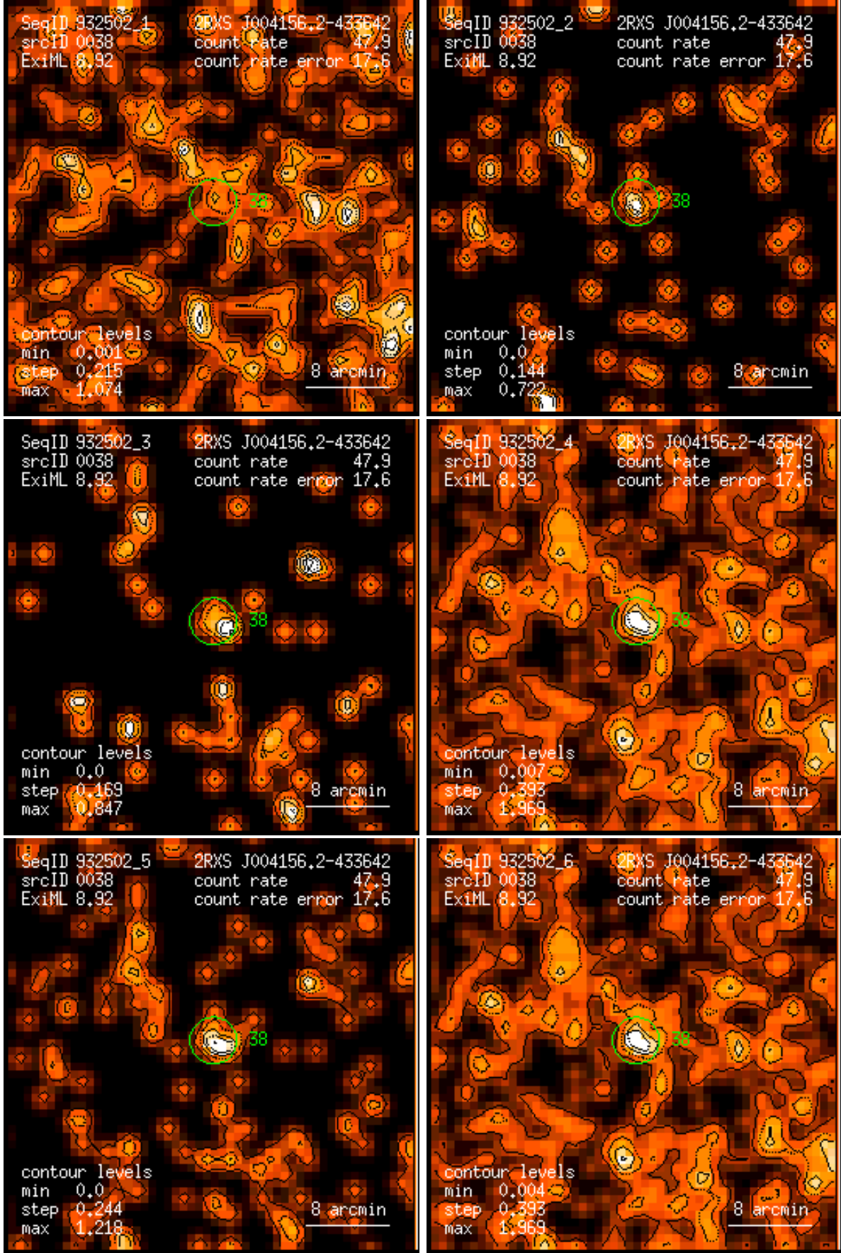
Figure 38: RASS 932502: detection 0038: band rate images, Gaussian filter: (1) PSPC channels 11 – 41, (2) 52 – 90, (3) 91 – 201, (4) 11 – 235, (5) 52 – 201, (6) 11 – 201. Broad band rates in counts/ks. Band rate contour levels in counts/ks/arcmin 2 .
