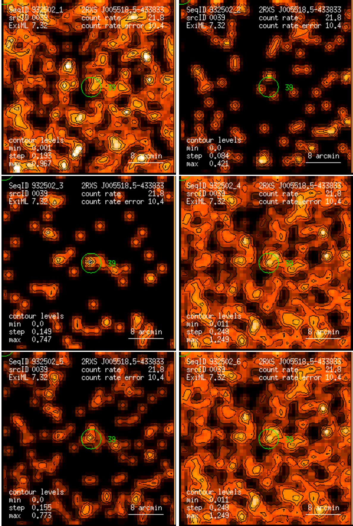
Figure 39: RASS 932502: detection 0039: band rate images, Gaussian filter: (1) PSPC channels 11 – 41, (2) 52 – 90, (3) 91 – 201, (4) 11 – 235, (5) 52 – 201, (6) 11 – 201. Broad band rates in counts/ks. Band rate contour levels in counts/ks/arcmin 2 .
