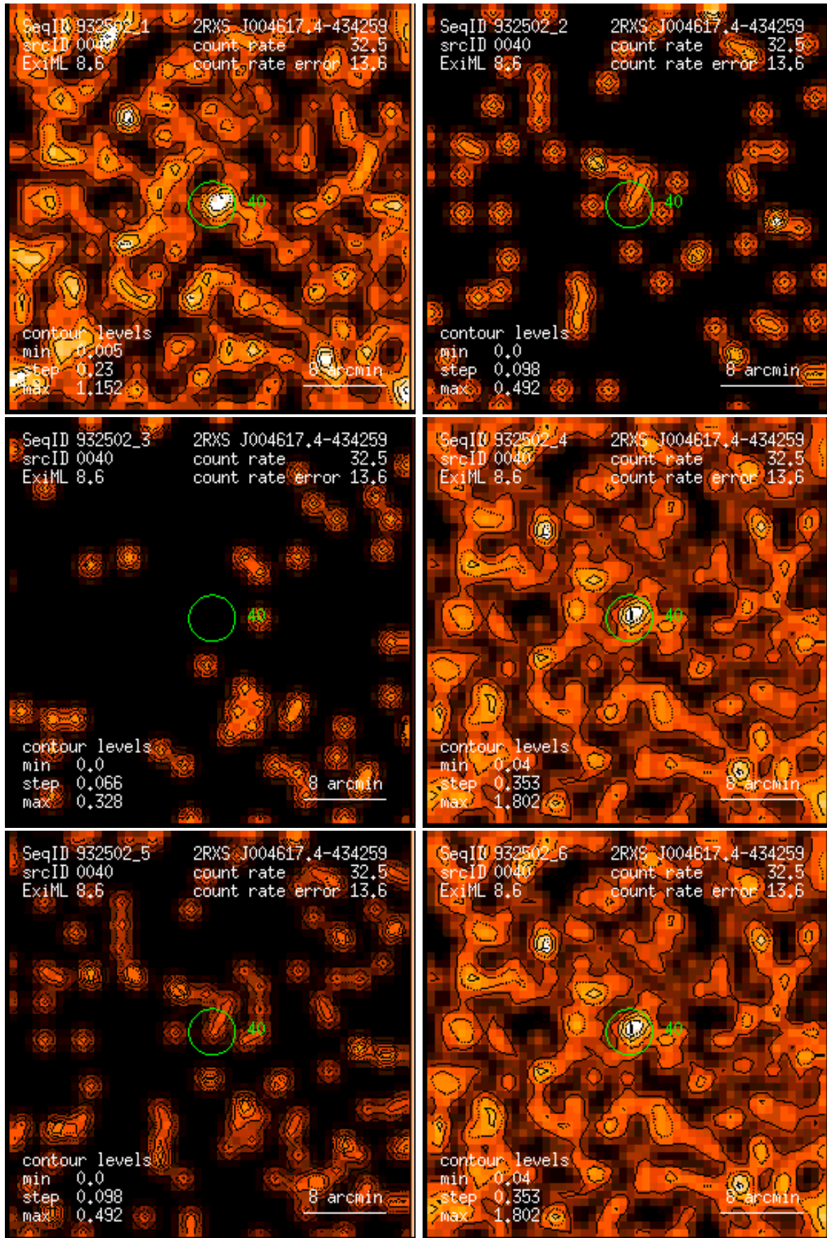
Figure 40: RASS 932502: detection 0040: band rate images, Gaussian filter: (1) PSPC channels 11 – 41, (2) 52 – 90, (3) 91 – 201, (4) 11 – 235, (5) 52 – 201, (6) 11 – 201. Broad band rates in counts/ks. Band rate contour levels in counts/ks/arcmin 2 .
