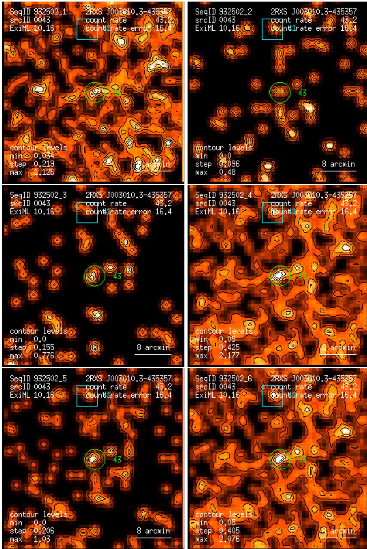
Figure 43: RASS 932502: detection 0043: band rate images, Gaussian filter: (1) PSPC channels 11 – 41, (2) 52 – 90, (3) 91 – 201, (4) 11 – 235, (5) 52 – 201, (6) 11 – 201. Broad band rates in counts/ks. Band rate contour levels in counts/ks/arcmin 2 .
