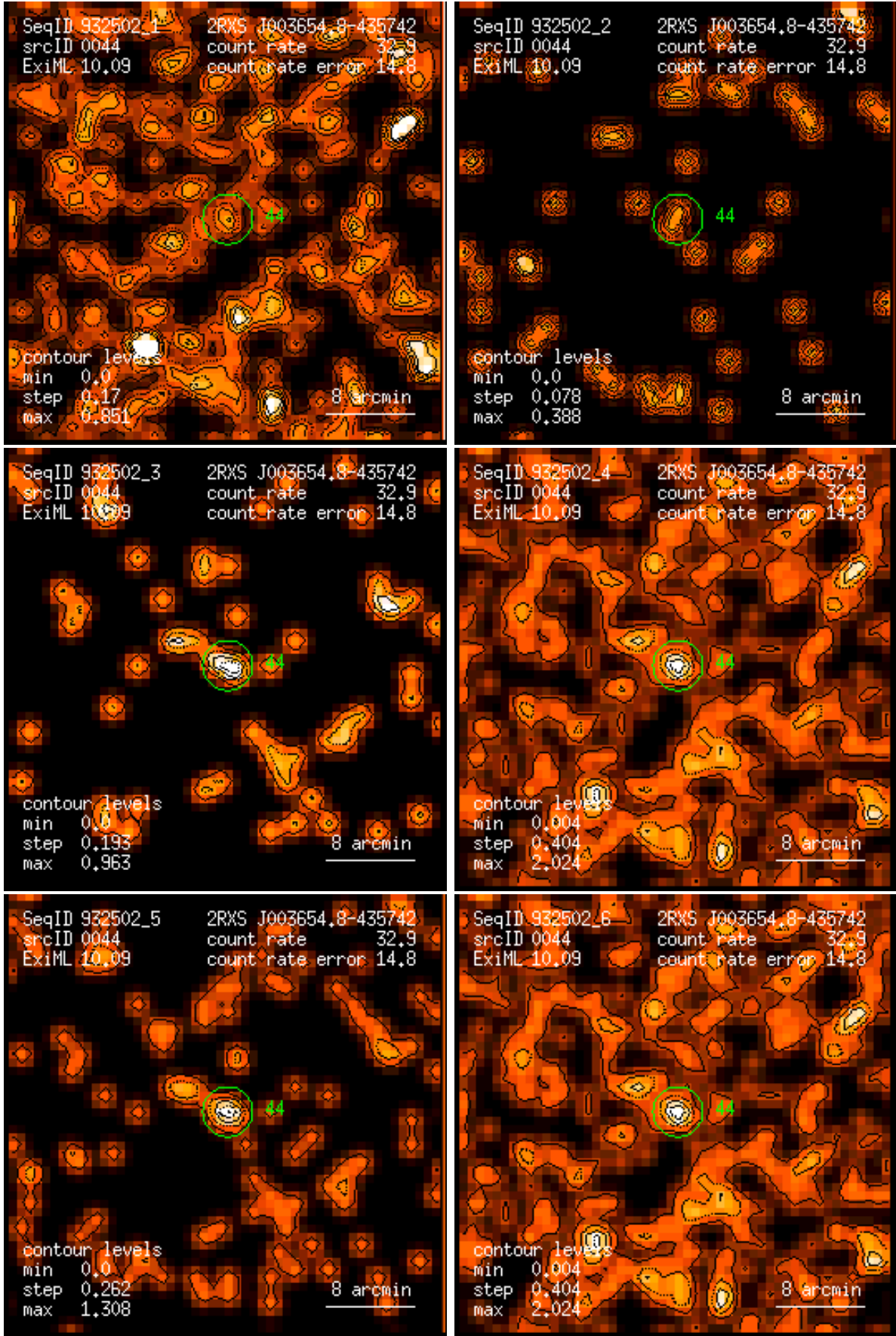
Figure 44: RASS 932502: detection 0044: band rate images, Gaussian filter: (1) PSPC channels 11 – 41, (2) 52 – 90, (3) 91 – 201, (4) 11 – 235, (5) 52 – 201, (6) 11 – 201. Broad band rates in counts/ks. Band rate contour levels in counts/ks/arcmin 2 .
