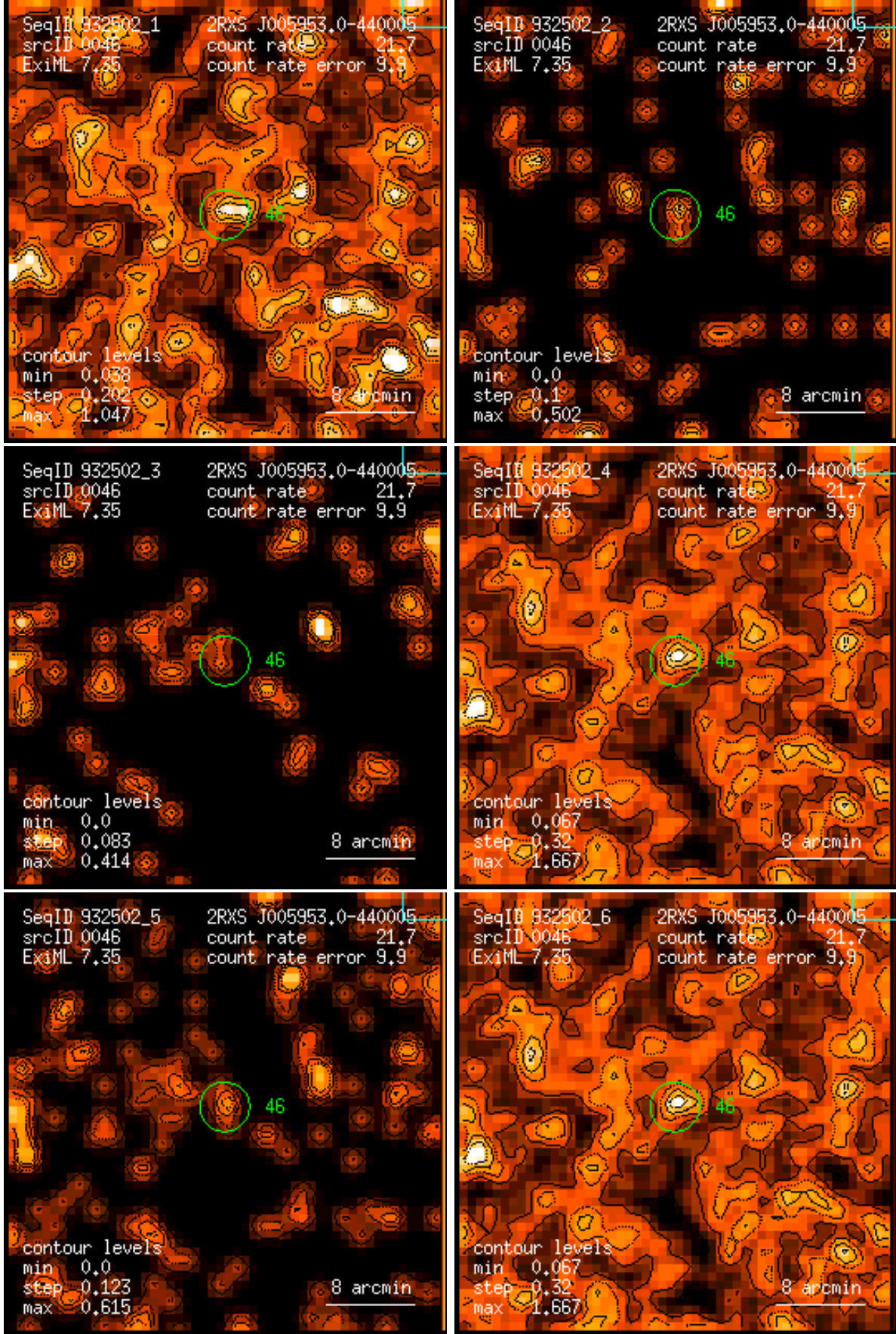
Figure 46: RASS 932502: detection 0046: band rate images, Gaussian filter: (1) PSPC channels 11 – 41, (2) 52 – 90, (3) 91 – 201, (4) 11 – 235, (5) 52 – 201, (6) 11 – 201. Broad band rates in counts/ks. Band rate contour levels in counts/ks/arcmin 2 .
