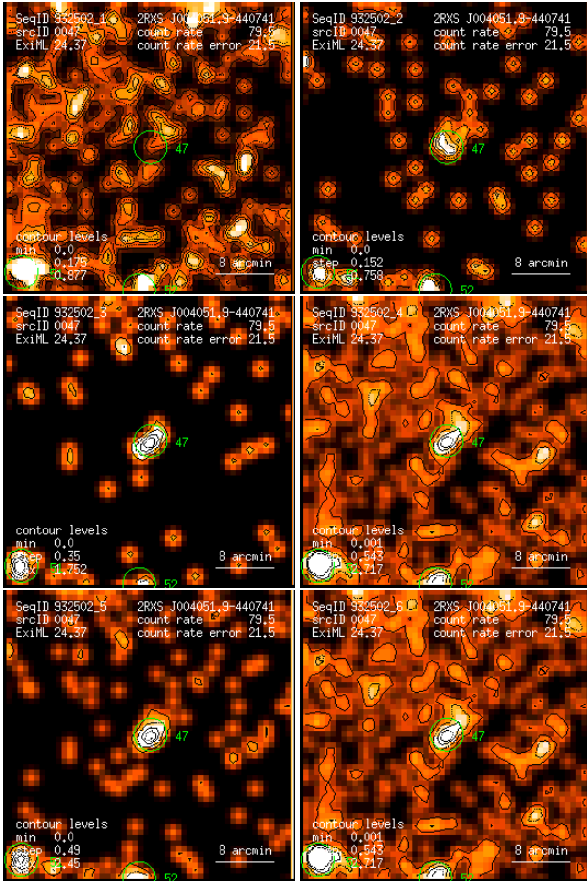
Figure 47: RASS 932502: detection 0047: band rate images, Gaussian filter: (1) PSPC channels 11 – 41, (2) 52 – 90, (3) 91 – 201, (4) 11 – 235, (5) 52 – 201, (6) 11 – 201. Broad band rates in counts/ks. Band rate contour levels in counts/ks/arcmin 2 .
