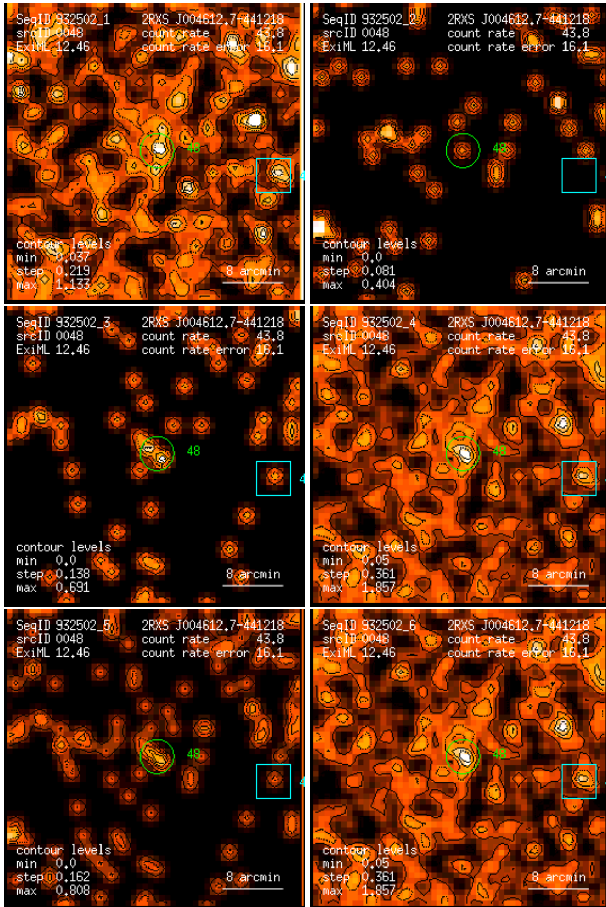
Figure 48: RASS 932502: detection 0048: band rate images, Gaussian filter: (1) PSPC channels 11 – 41, (2) 52 – 90, (3) 91 – 201, (4) 11 – 235, (5) 52 – 201, (6) 11 – 201. Broad band rates in counts/ks. Band rate contour levels in counts/ks/arcmin 2 .
