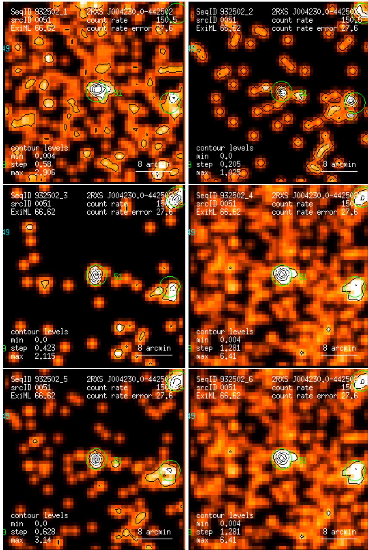
Figure 51: RASS 932502: detection 0051: band rate images, Gaussian filter: (1) PSPC channels 11 – 41, (2) 52 – 90, (3) 91 – 201, (4) 11 – 235, (5) 52 – 201, (6) 11 – 201. Broad band rates in counts/ks. Band rate contour levels in counts/ks/arcmin 2 .
