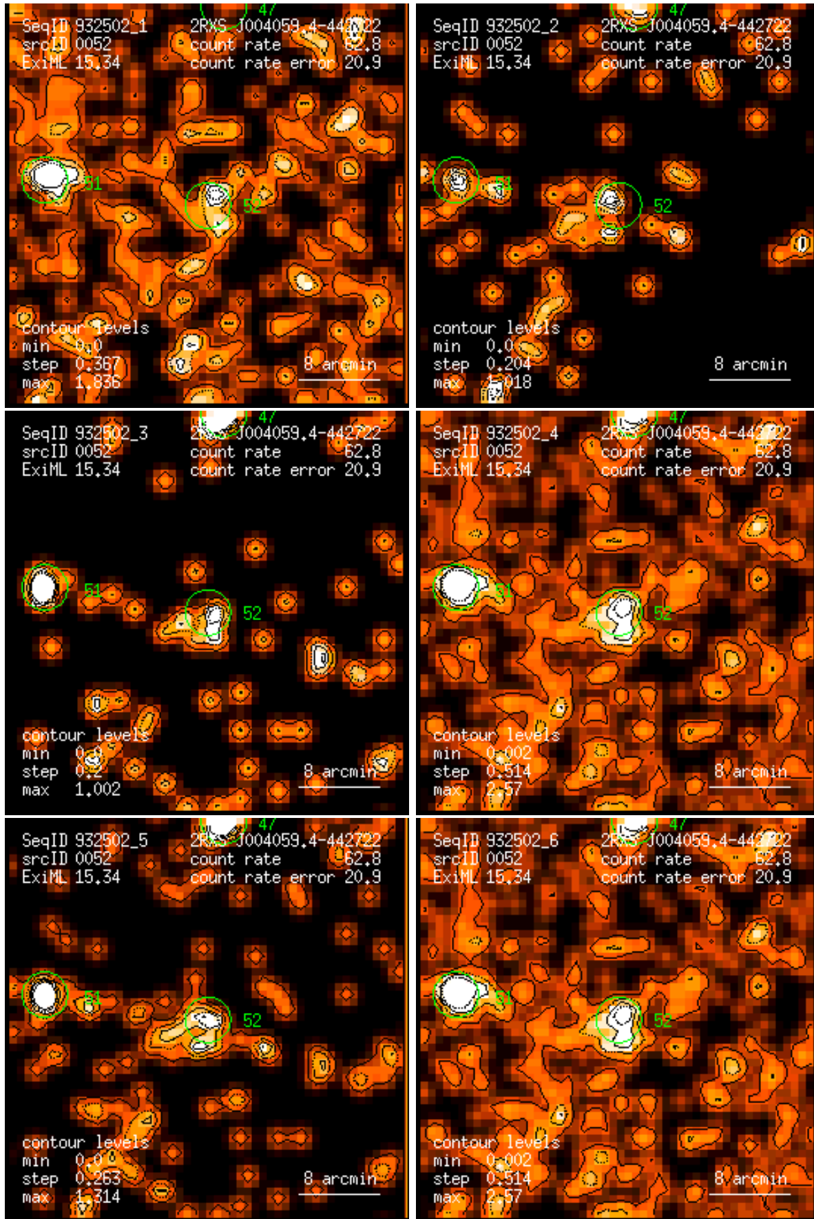
Figure 52: RASS 932502: detection 0052: band rate images, Gaussian filter: (1) PSPC channels 11 – 41, (2) 52 – 90, (3) 91 – 201, (4) 11 – 235, (5) 52 – 201, (6) 11 – 201. Broad band rates in counts/ks. Band rate contour levels in counts/ks/arcmin 2 .
