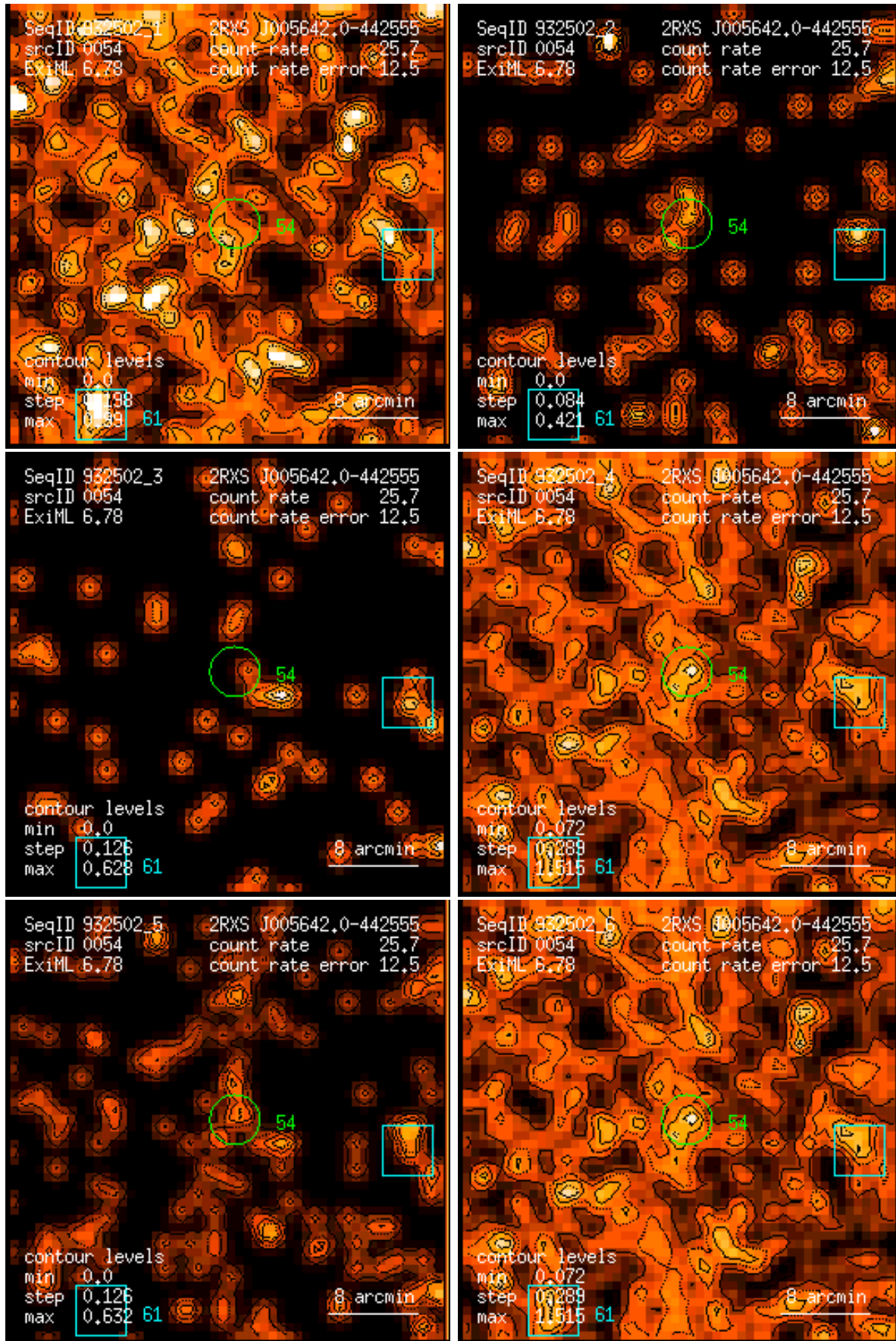
Figure 54: RASS 932502: detection 0054: band rate images, Gaussian filter: (1) PSPC channels 11 – 41, (2) 52 – 90, (3) 91 – 201, (4) 11 – 235, (5) 52 – 201, (6) 11 – 201. Broad band rates in counts/ks. Band rate contour levels in counts/ks/arcmin 2 .
