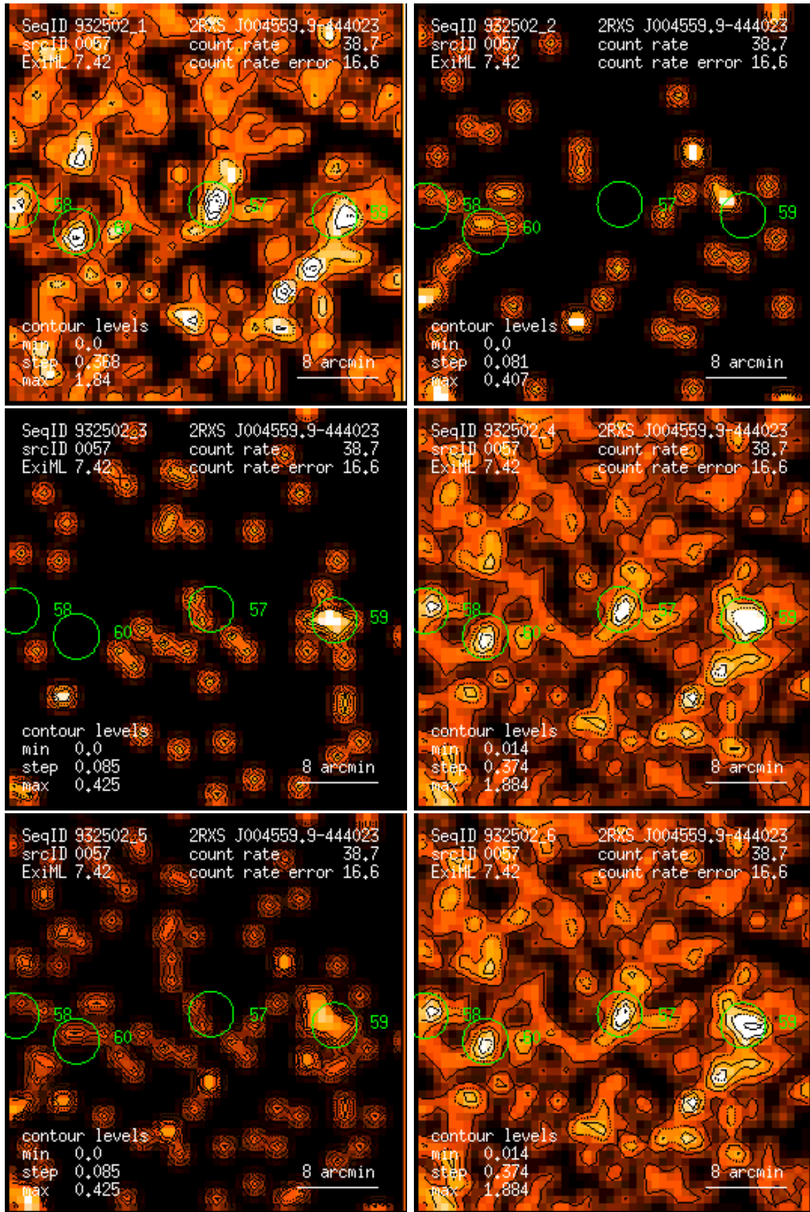
Figure 57: RASS 932502: detection 0057: band rate images, Gaussian filter: (1) PSPC channels 11 – 41, (2) 52 – 90, (3) 91 – 201, (4) 11 – 235, (5) 52 – 201, (6) 11 – 201. Broad band rates in counts/ks. Band rate contour levels in counts/ks/arcmin 2 .
