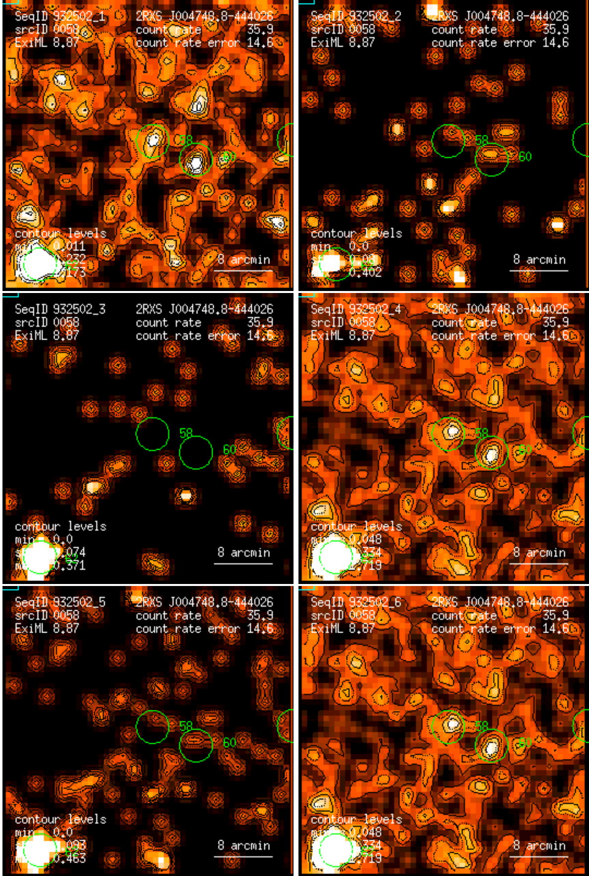
Figure 58: RASS 932502: detection 0058: band rate images, Gaussian filter: (1) PSPC channels 11 – 41, (2) 52 – 90, (3) 91 – 201, (4) 11 – 235, (5) 52 – 201, (6) 11 – 201. Broad band rates in counts/ks. Band rate contour levels in counts/ks/arcmin 2 .
