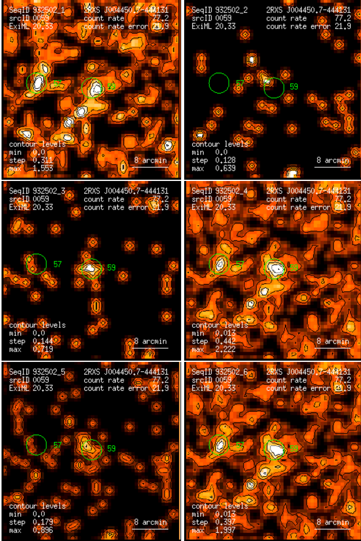
Figure 59: RASS 932502: detection 0059: band rate images, Gaussian filter: (1) PSPC channels 11 – 41, (2) 52 – 90, (3) 91 – 201, (4) 11 – 235, (5) 52 – 201, (6) 11 – 201. Broad band rates in counts/ks. Band rate contour levels in counts/ks/arcmin 2 .
