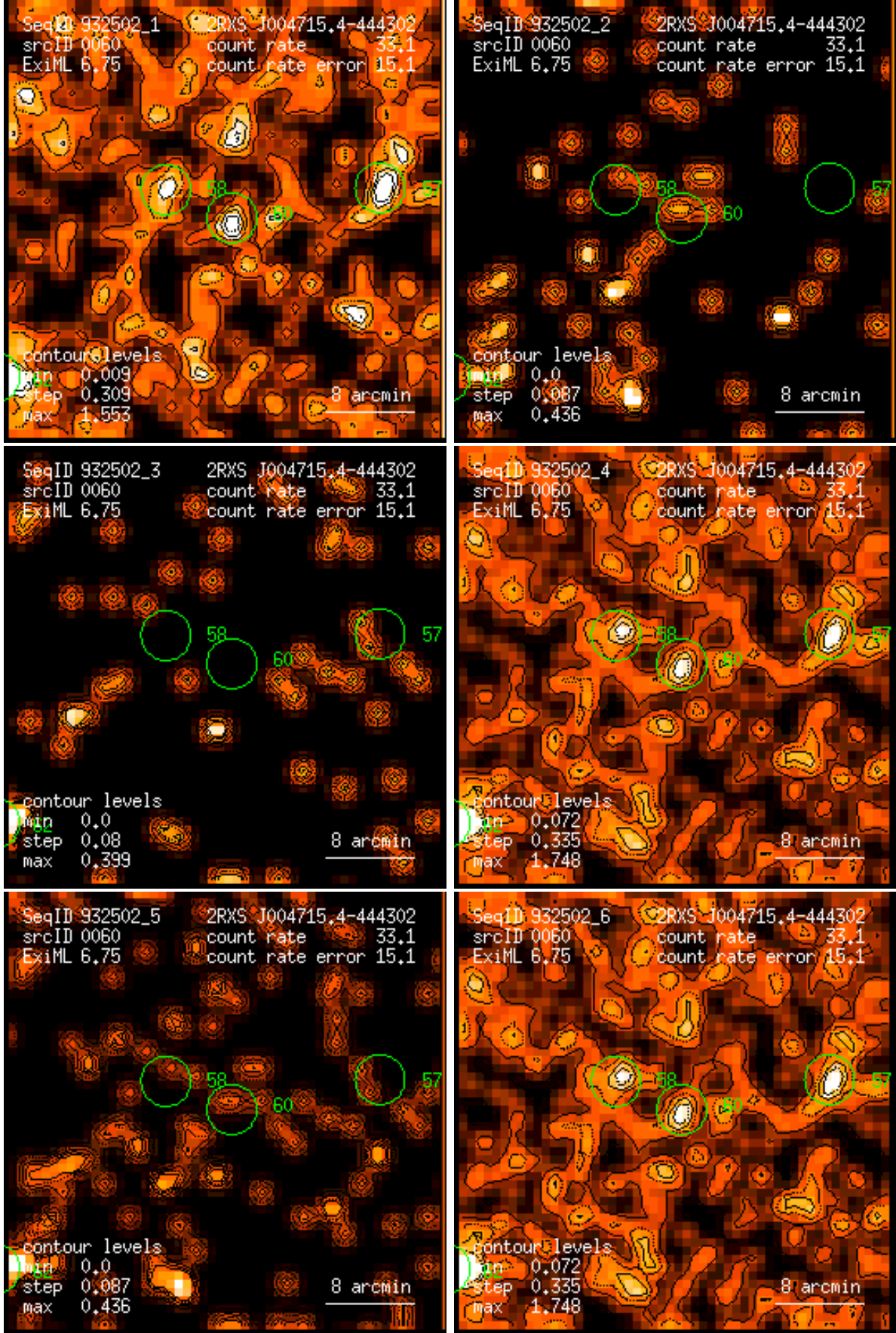
Figure 60: RASS 932502: detection 0060: band rate images, Gaussian filter: (1) PSPC channels 11 – 41, (2) 52 – 90, (3) 91 – 201, (4) 11 – 235, (5) 52 – 201, (6) 11 – 201. Broad band rates in counts/ks. Band rate contour levels in counts/ks/arcmin 2 .
