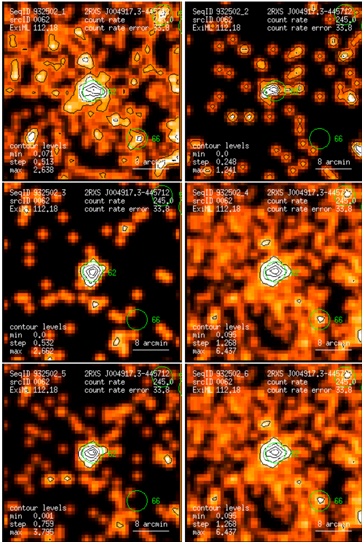
Figure 62: RASS 932502: detection 0062: band rate images, Gaussian filter: (1) PSPC channels 11 – 41, (2) 52 – 90, (3) 91 – 201, (4) 11 – 235, (5) 52 – 201, (6) 11 – 201. Broad band rates in counts/ks. Band rate contour levels in counts/ks/arcmin 2 .
