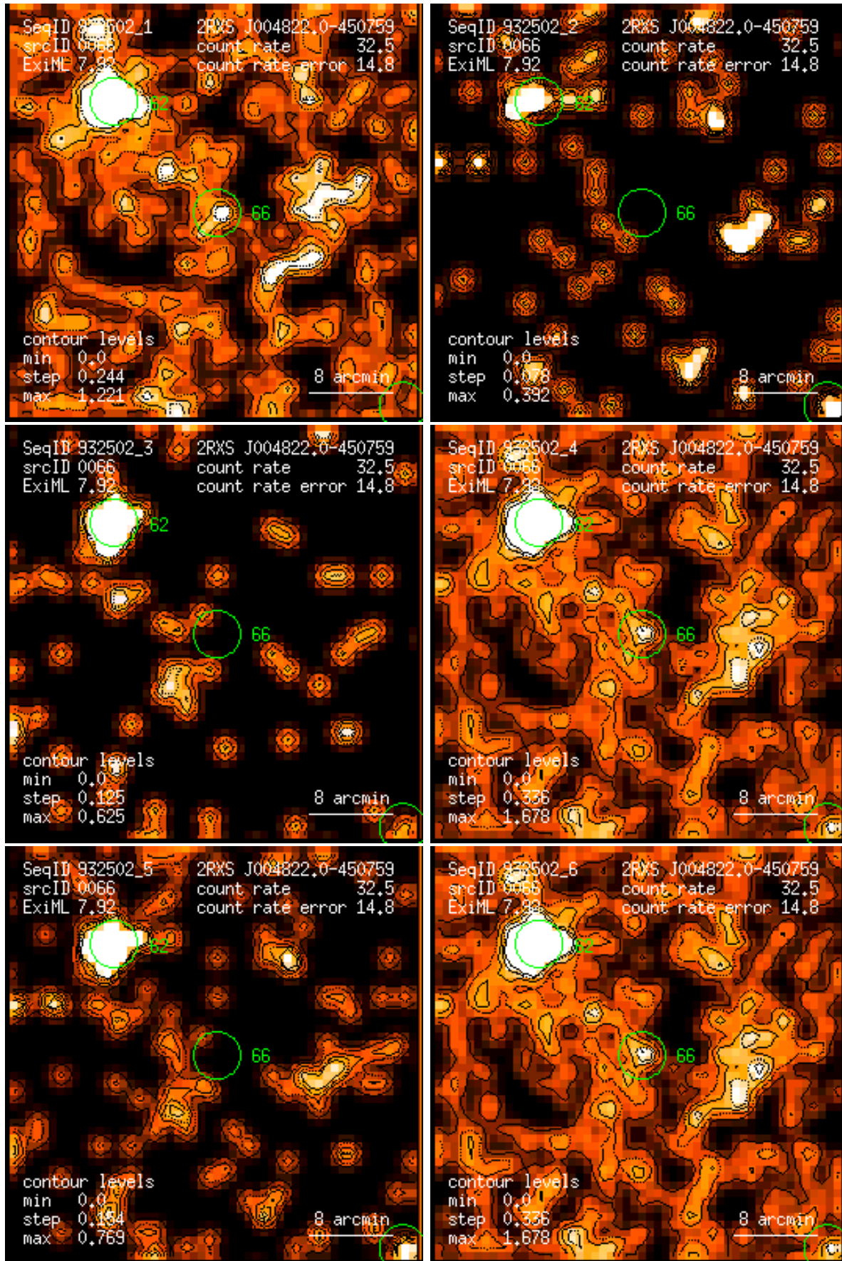
Figure 66: RASS 932502: detection 0066: band rate images, Gaussian filter: (1) PSPC channels 11 – 41, (2) 52 – 90, (3) 91 – 201, (4) 11 – 235, (5) 52 – 201, (6) 11 – 201. Broad band rates in counts/ks. Band rate contour levels in counts/ks/arcmin 2 .
