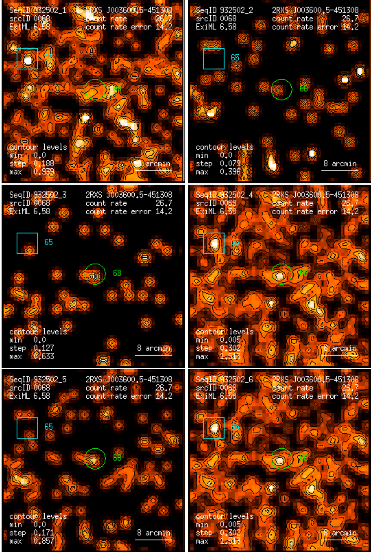
Figure 68: RASS 932502: detection 0068: band rate images, Gaussian filter: (1) PSPC channels 11 – 41, (2) 52 – 90, (3) 91 – 201, (4) 11 – 235, (5) 52 – 201, (6) 11 – 201. Broad band rates in counts/ks. Band rate contour levels in counts/ks/arcmin 2 .
