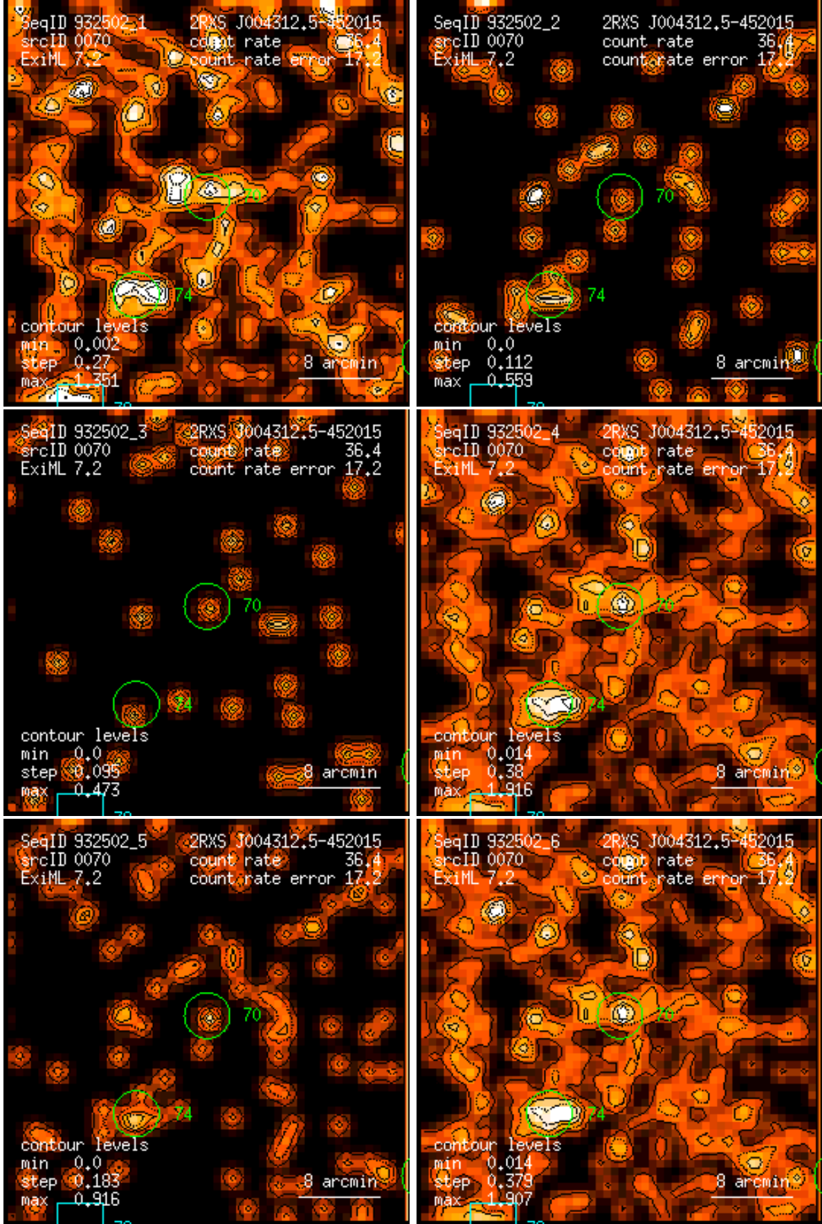
Figure 70: RASS 932502: detection 0070: band rate images, Gaussian filter: (1) PSPC channels 11 – 41, (2) 52 – 90, (3) 91 – 201, (4) 11 – 235, (5) 52 – 201, (6) 11 – 201. Broad band rates in counts/ks. Band rate contour levels in counts/ks/arcmin 2 .
