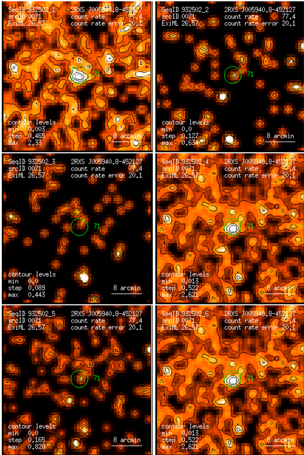
Figure 71: RASS 932502: detection 0071: band rate images, Gaussian filter: (1) PSPC channels 11 – 41, (2) 52 – 90, (3) 91 – 201, (4) 11 – 235, (5) 52 – 201, (6) 11 – 201. Broad band rates in counts/ks. Band rate contour levels in counts/ks/arcmin 2 .
