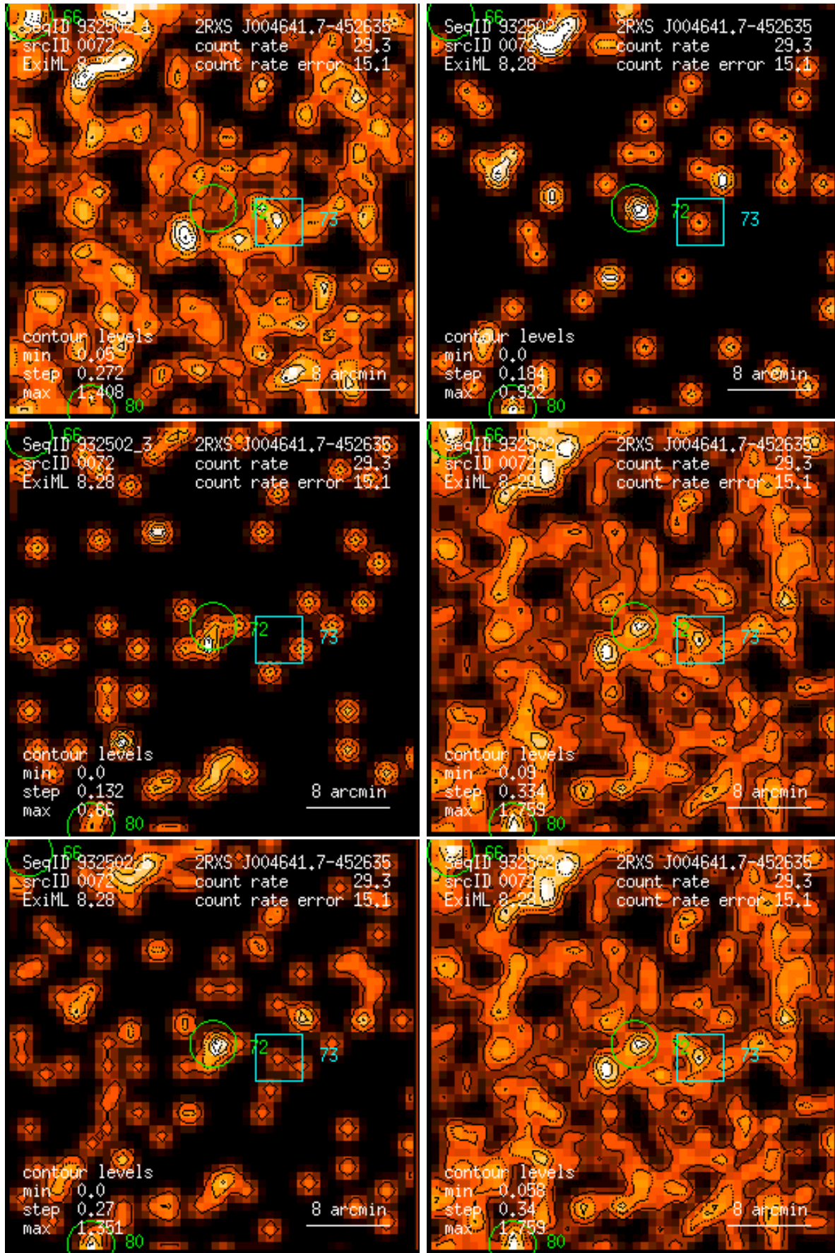
Figure 72: RASS 932502: detection 0072: band rate images, Gaussian filter: (1) PSPC channels 11 – 41, (2) 52 – 90, (3) 91 – 201, (4) 11 – 235, (5) 52 – 201, (6) 11 – 201. Broad band rates in counts/ks. Band rate contour levels in counts/ks/arcmin 2 .
