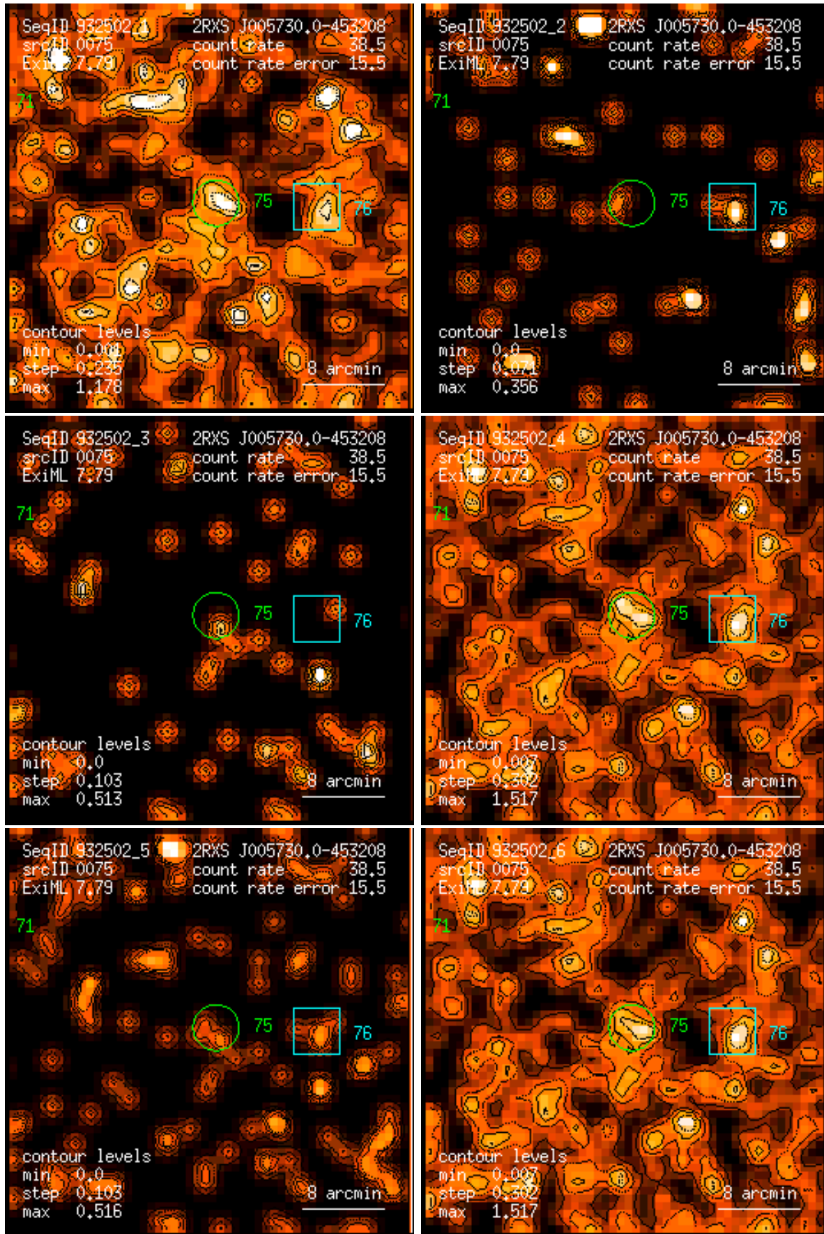
Figure 75: RASS 932502: detection 0075: band rate images, Gaussian filter: (1) PSPC channels 11 – 41, (2) 52 – 90, (3) 91 – 201, (4) 11 – 235, (5) 52 – 201, (6) 11 – 201. Broad band rates in counts/ks. Band rate contour levels in counts/ks/arcmin 2 .
