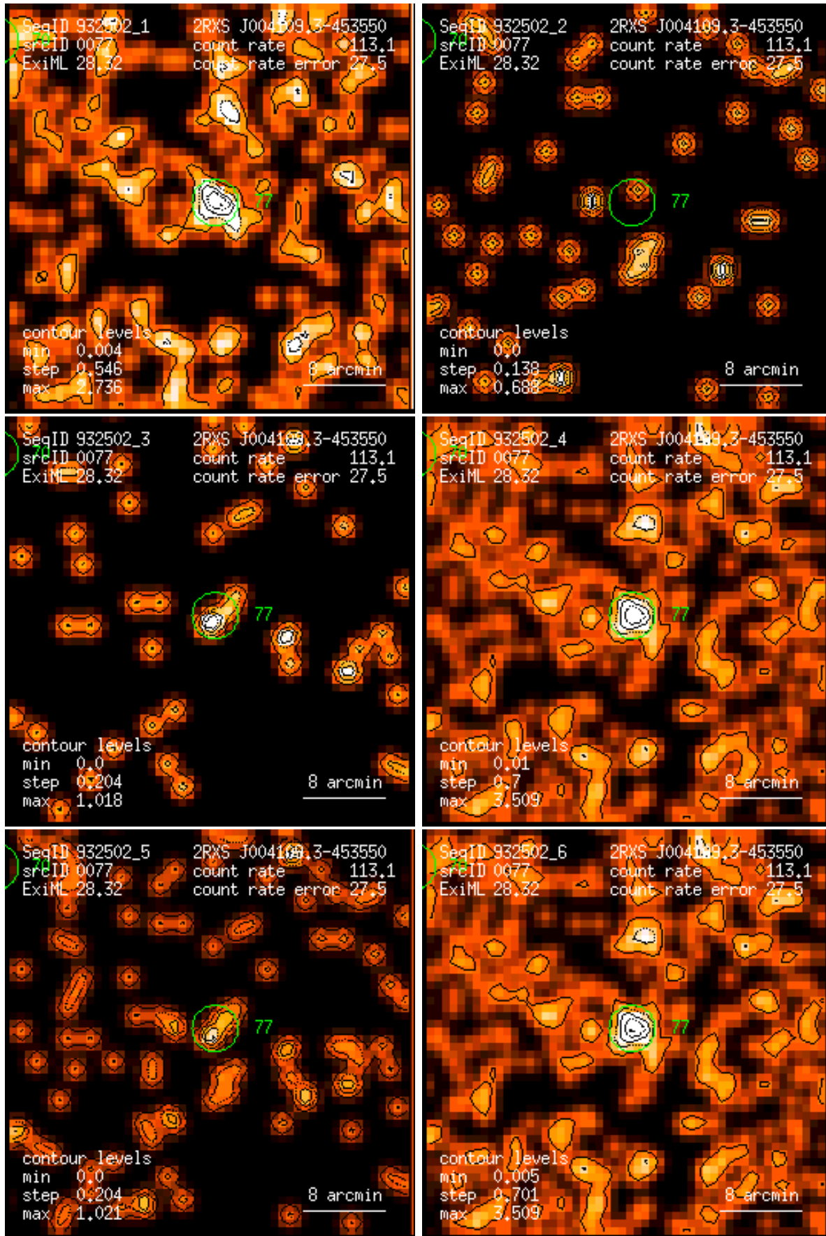
Figure 77: RASS 932502: detection 0077: band rate images, Gaussian filter: (1) PSPC channels 11 – 41, (2) 52 – 90, (3) 91 – 201, (4) 11 – 235, (5) 52 – 201, (6) 11 – 201. Broad band rates in counts/ks. Band rate contour levels in counts/ks/arcmin 2 .
