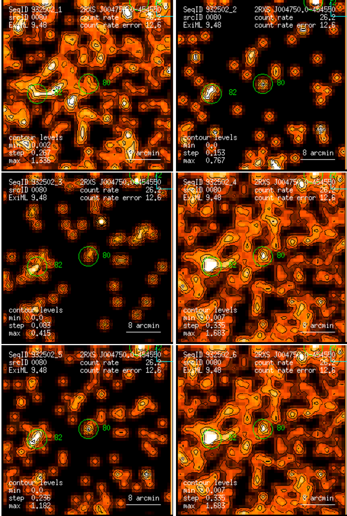
Figure 80: RASS 932502: detection 0080: band rate images, Gaussian filter: (1) PSPC channels 11 – 41, (2) 52 – 90, (3) 91 – 201, (4) 11 – 235, (5) 52 – 201, (6) 11 – 201. Broad band rates in counts/ks. Band rate contour levels in counts/ks/arcmin 2 .
