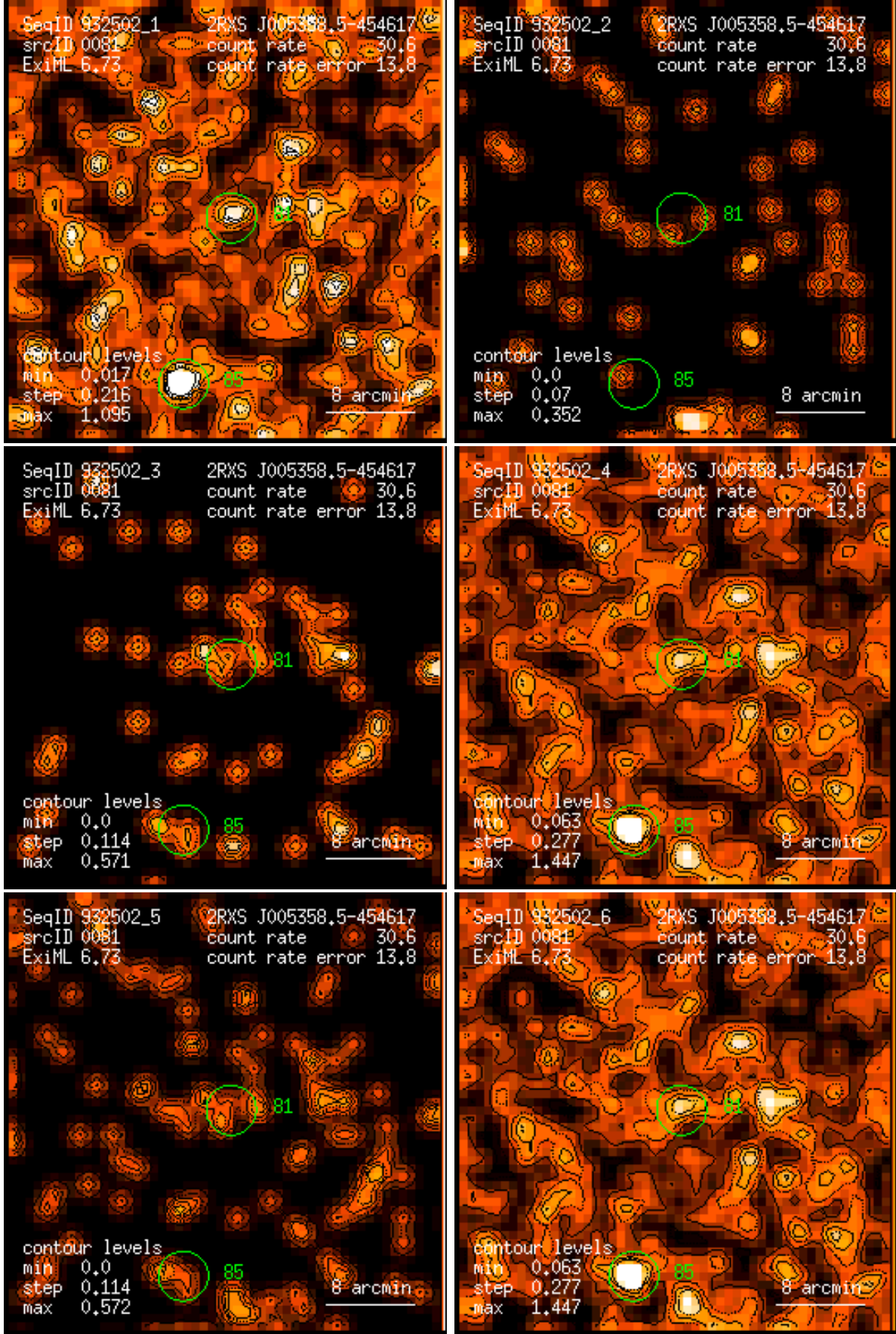
Figure 81: RASS 932502: detection 0081: band rate images, Gaussian filter: (1) PSPC channels 11 – 41, (2) 52 – 90, (3) 91 – 201, (4) 11 – 235, (5) 52 – 201, (6) 11 – 201. Broad band rates in counts/ks. Band rate contour levels in counts/ks/arcmin 2 .
