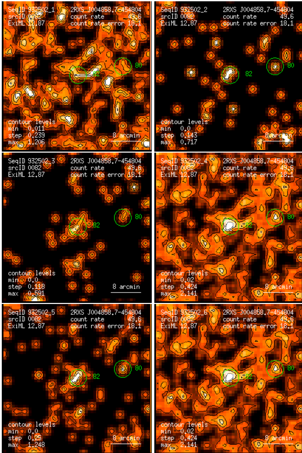
Figure 82: RASS 932502: detection 0082: band rate images, Gaussian filter: (1) PSPC channels 11 – 41, (2) 52 – 90, (3) 91 – 201, (4) 11 – 235, (5) 52 – 201, (6) 11 – 201. Broad band rates in counts/ks. Band rate contour levels in counts/ks/arcmin 2 .
