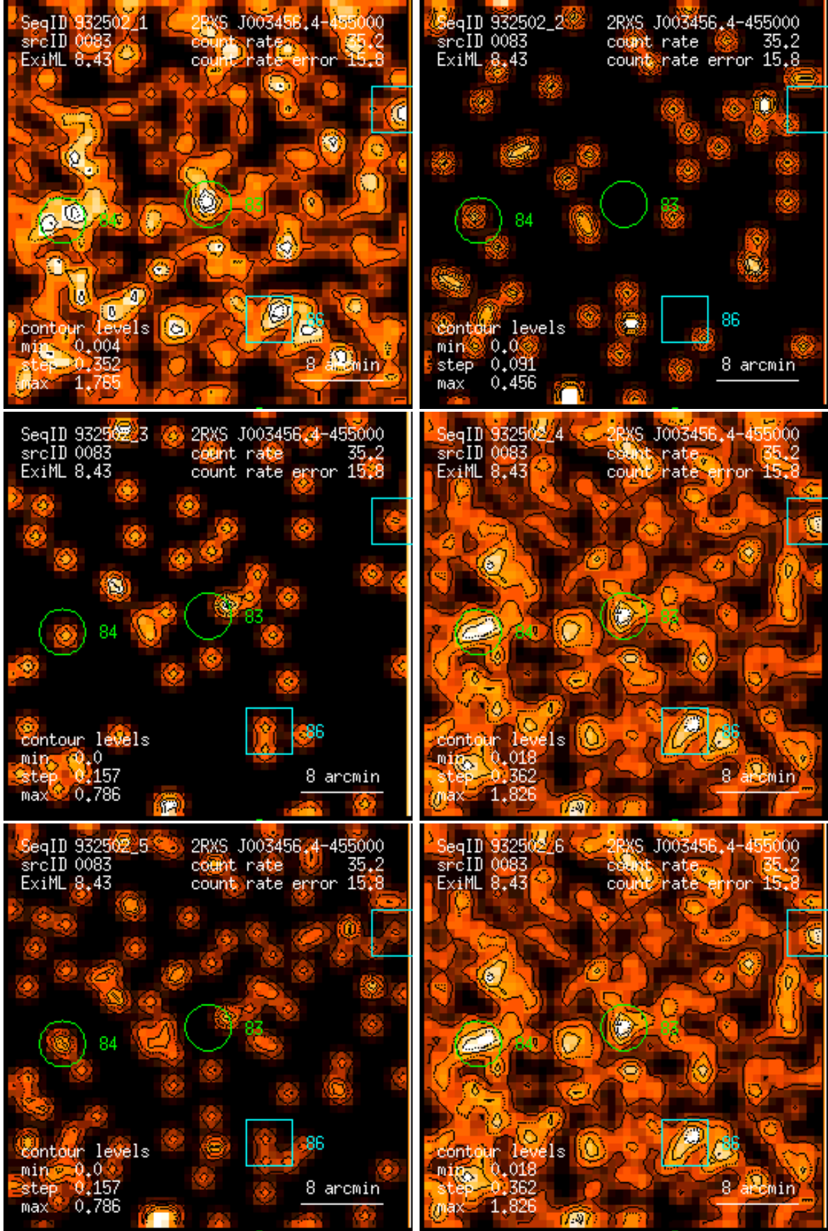
Figure 83: RASS 932502: detection 0083: band rate images, Gaussian filter: (1) PSPC channels 11 – 41, (2) 52 – 90, (3) 91 – 201, (4) 11 – 235, (5) 52 – 201, (6) 11 – 201. Broad band rates in counts/ks. Band rate contour levels in counts/ks/arcmin 2 .
