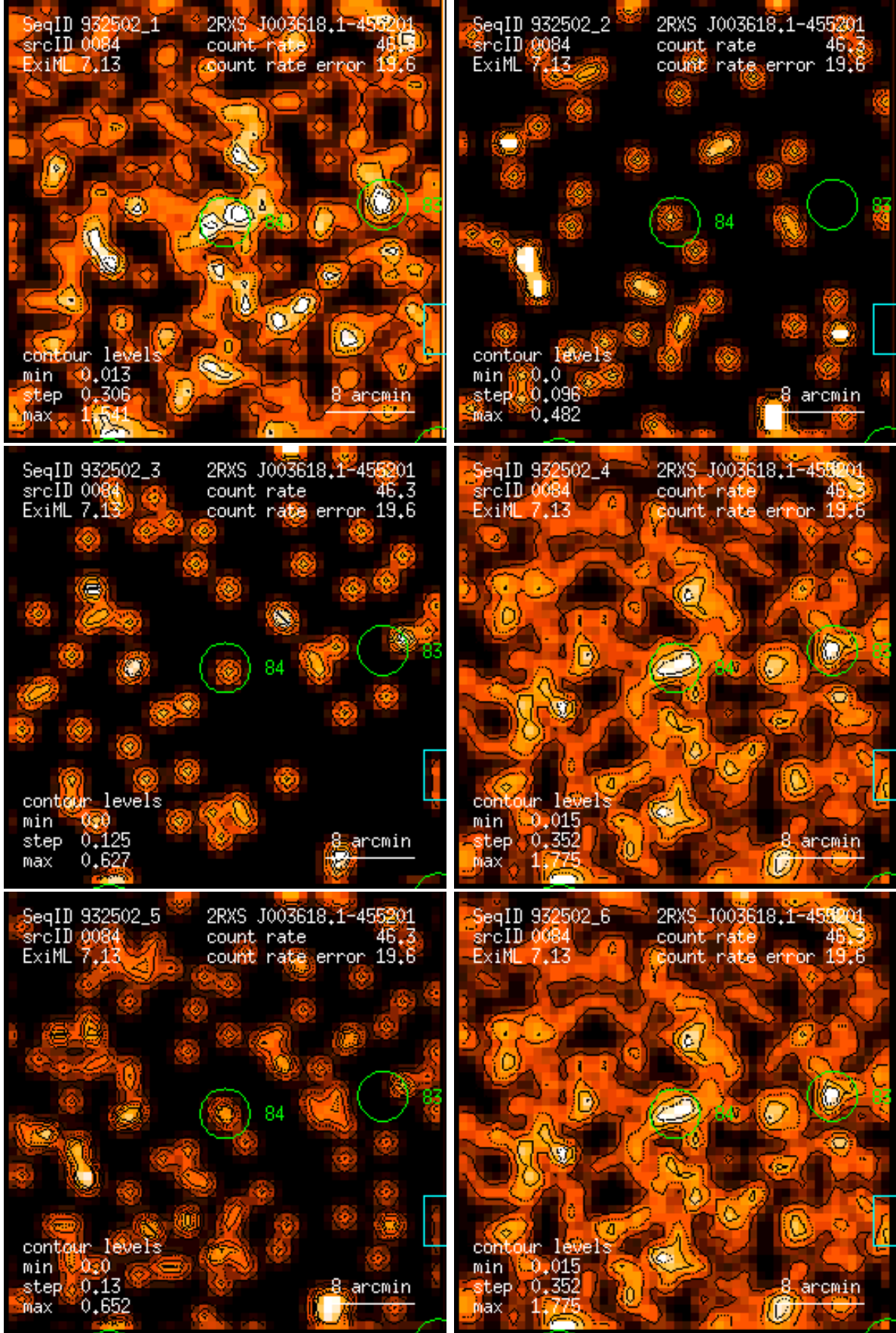
Figure 84: RASS 932502: detection 0084: band rate images, Gaussian filter: (1) PSPC channels 11 – 41, (2) 52 – 90, (3) 91 – 201, (4) 11 – 235, (5) 52 – 201, (6) 11 – 201. Broad band rates in counts/ks. Band rate contour levels in counts/ks/arcmin 2 .
