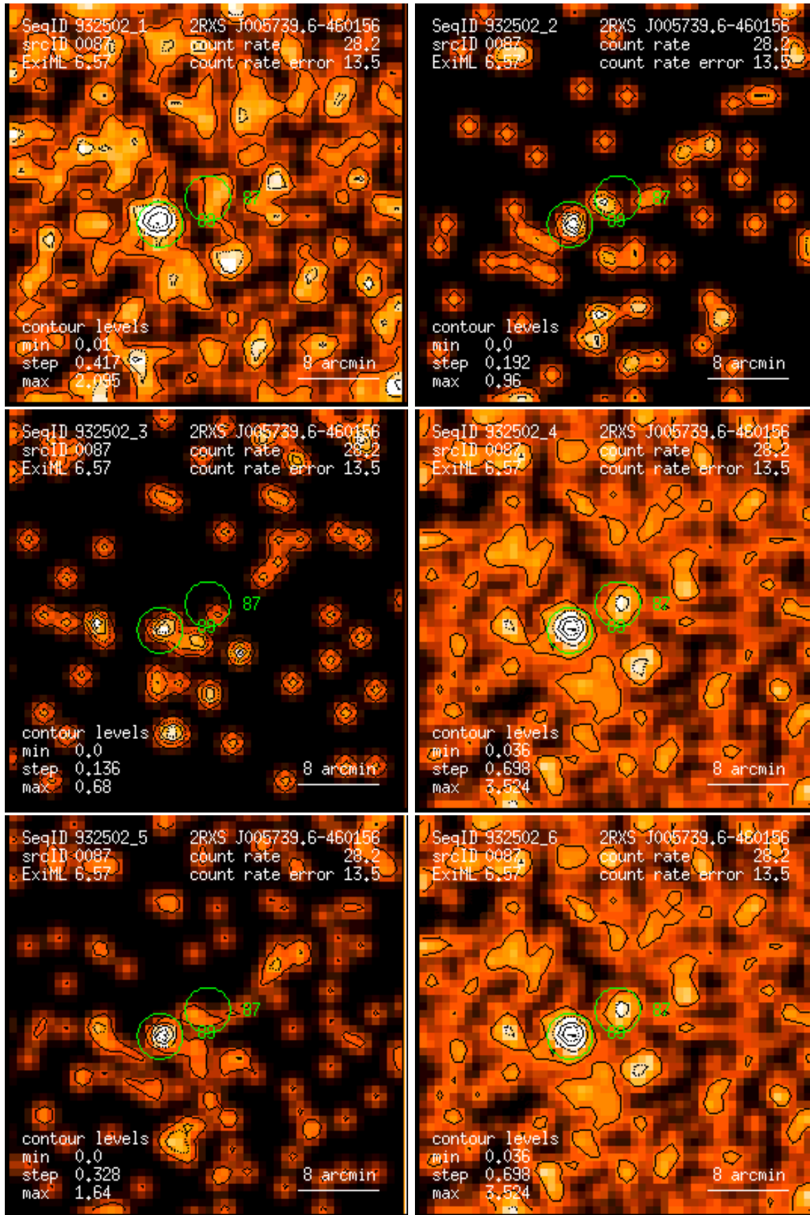
Figure 87: RASS 932502: detection 0087: band rate images, Gaussian filter: (1) PSPC channels 11 – 41, (2) 52 – 90, (3) 91 – 201, (4) 11 – 235, (5) 52 – 201, (6) 11 – 201. Broad band rates in counts/ks. Band rate contour levels in counts/ks/arcmin 2 .
