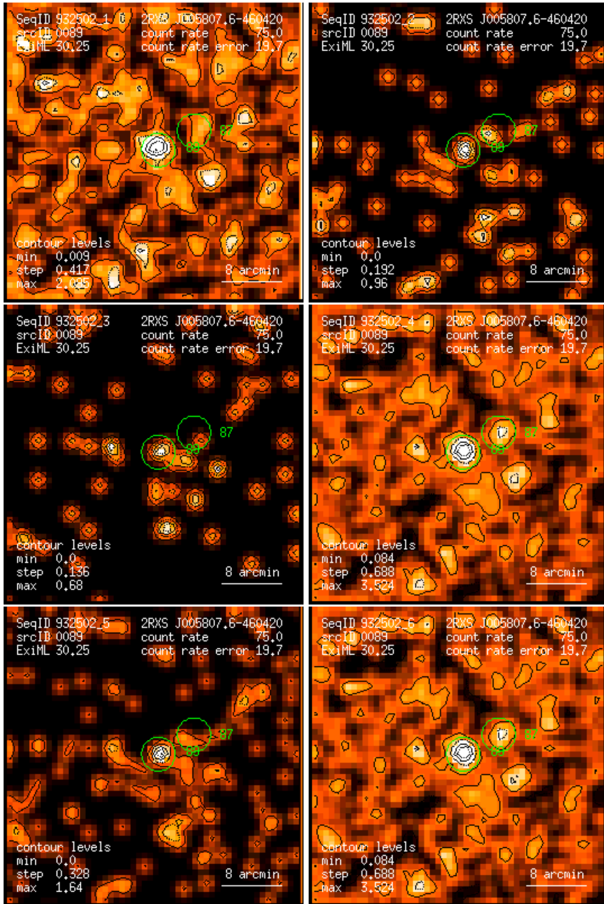
Figure 89: RASS 932502: detection 0089: band rate images, Gaussian filter: (1) PSPC channels 11 – 41, (2) 52 – 90, (3) 91 – 201, (4) 11 – 235, (5) 52 – 201, (6) 11 – 201. Broad band rates in counts/ks. Band rate contour levels in counts/ks/arcmin 2 .
