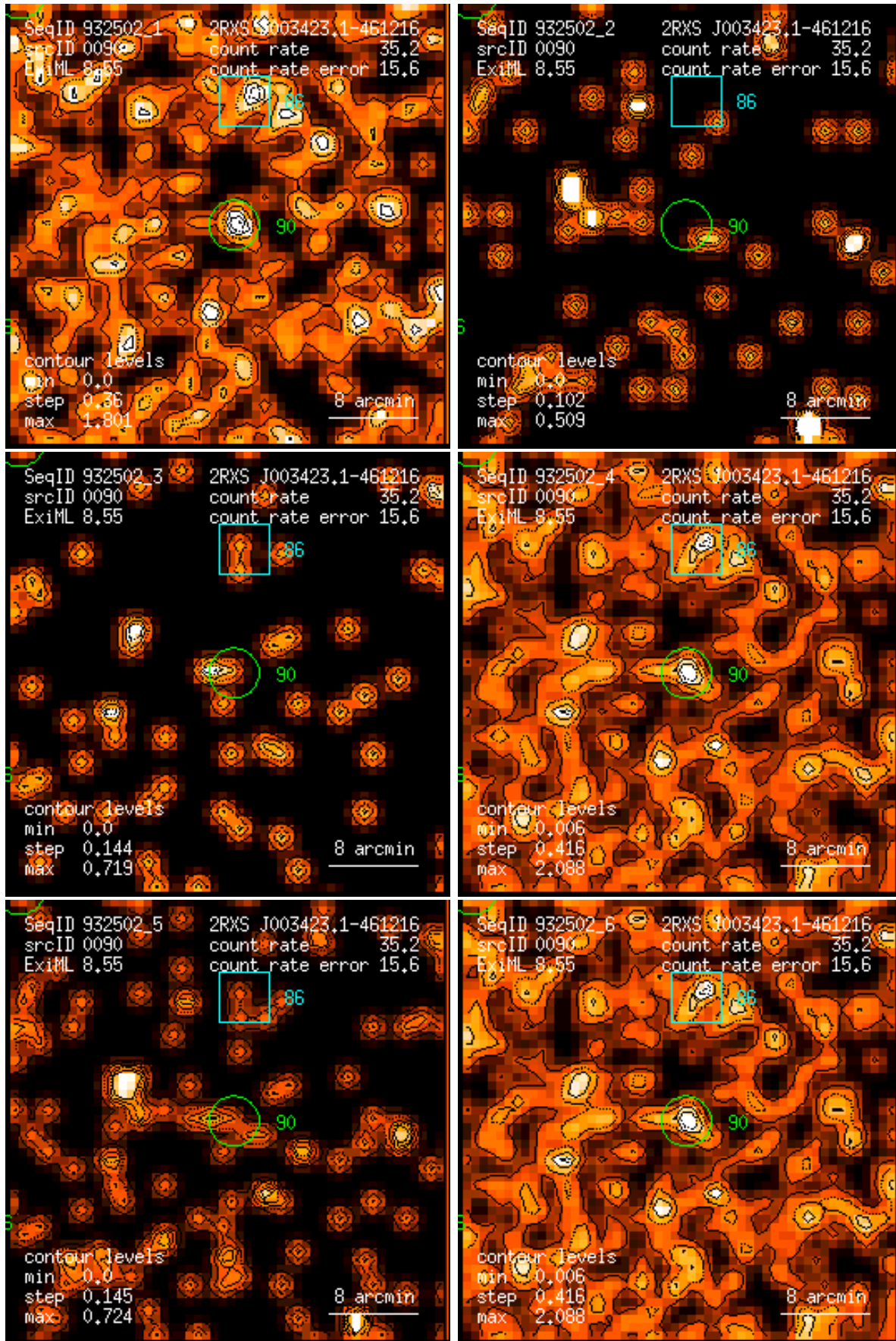
Figure 90: RASS 932502: detection 0090: band rate images, Gaussian filter: (1) PSPC channels 11 – 41, (2) 52 – 90, (3) 91 – 201, (4) 11 – 235, (5) 52 – 201, (6) 11 – 201. Broad band rates in counts/ks. Band rate contour levels in counts/ks/arcmin 2 .
