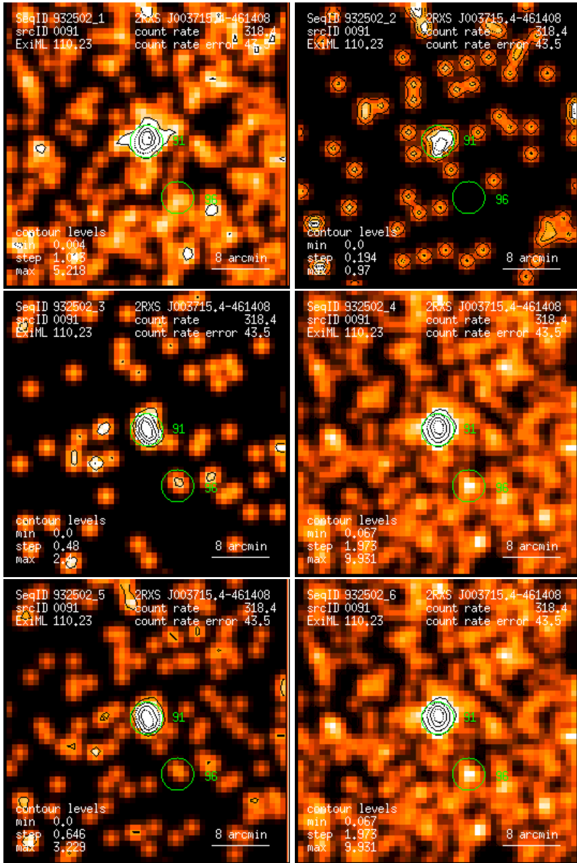
Figure 91: RASS 932502: detection 0091: band rate images, Gaussian filter: (1) PSPC channels 11 – 41, (2) 52 – 90, (3) 91 – 201, (4) 11 – 235, (5) 52 – 201, (6) 11 – 201. Broad band rates in counts/ks. Band rate contour levels in counts/ks/arcmin 2 .
