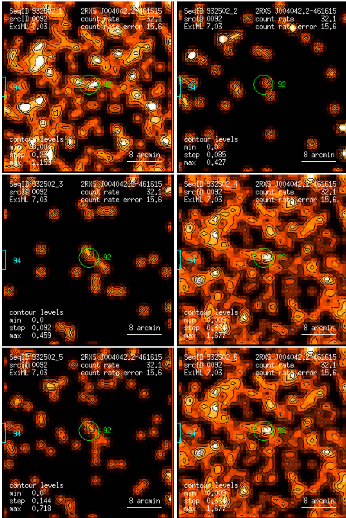
Figure 92: RASS 932502: detection 0092: band rate images, Gaussian filter: (1) PSPC channels 11 – 41, (2) 52 – 90, (3) 91 – 201, (4) 11 – 235, (5) 52 – 201, (6) 11 – 201. Broad band rates in counts/ks. Band rate contour levels in counts/ks/arcmin 2 .
