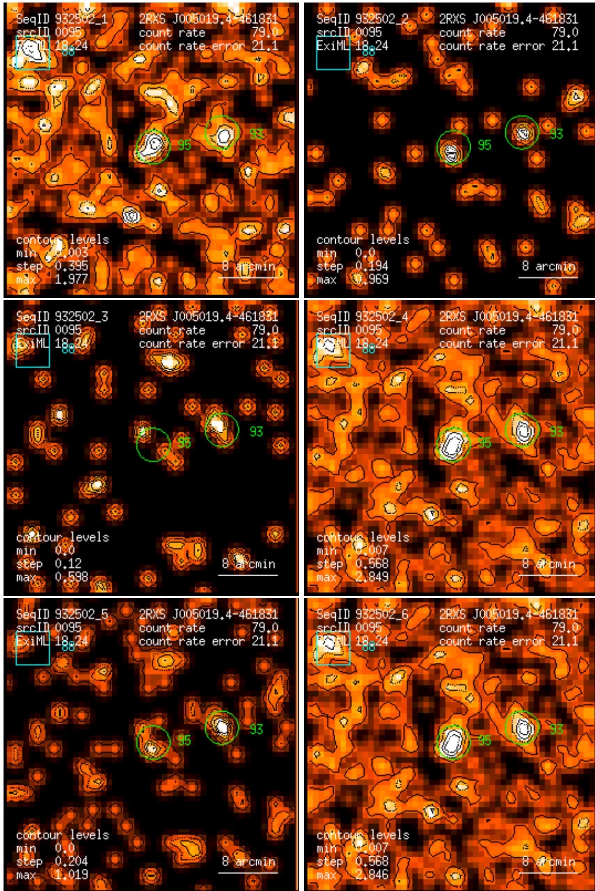
Figure 95: RASS 932502: detection 0095: band rate images, Gaussian filter: (1) PSPC channels 11 – 41, (2) 52 – 90, (3) 91 – 201, (4) 11 – 235, (5) 52 – 201, (6) 11 – 201. Broad band rates in counts/ks. Band rate contour levels in counts/ks/arcmin 2 .
