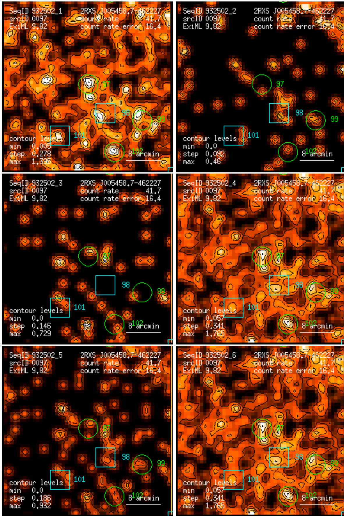
Figure 97: RASS 932502: detection 0097: band rate images, Gaussian filter: (1) PSPC channels 11 – 41, (2) 52 – 90, (3) 91 – 201, (4) 11 – 235, (5) 52 – 201, (6) 11 – 201. Broad band rates in counts/ks. Band rate contour levels in counts/ks/arcmin 2 .
